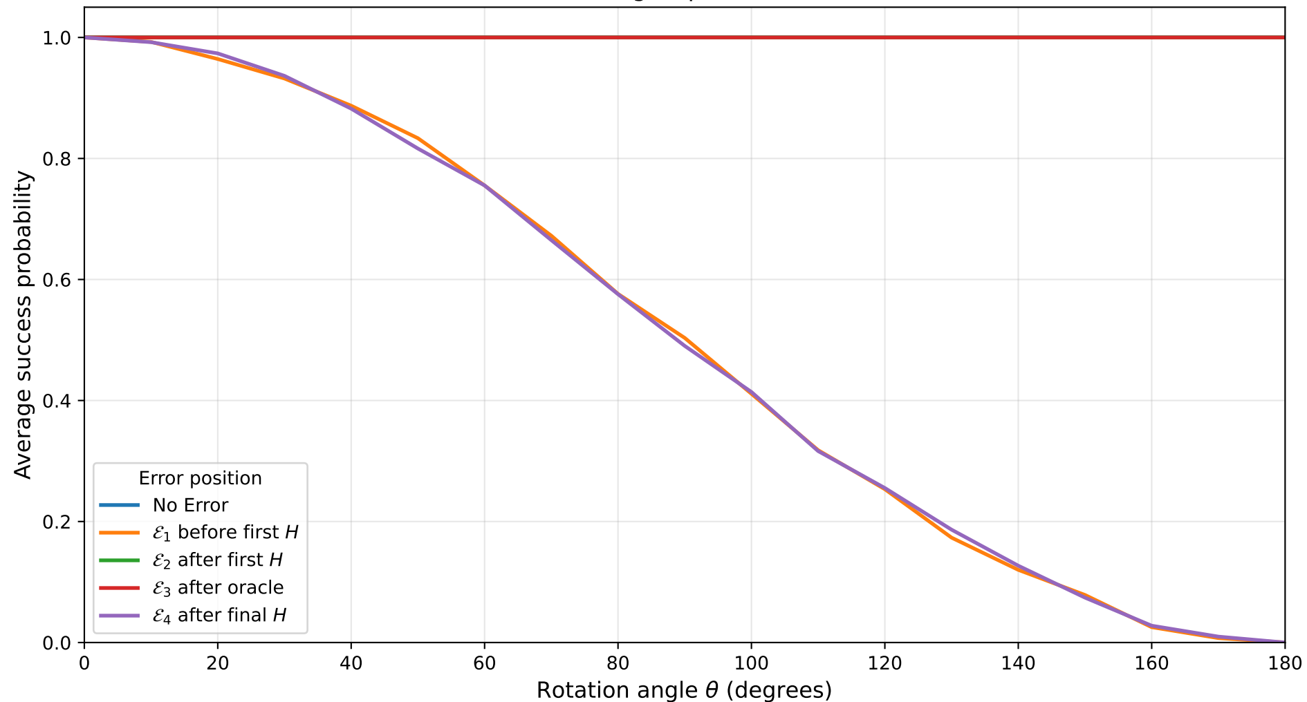
Deutsch-Jozsa Algorithm under Rotation Errors n=1, axis=X, target qubit=0, shots=1024
