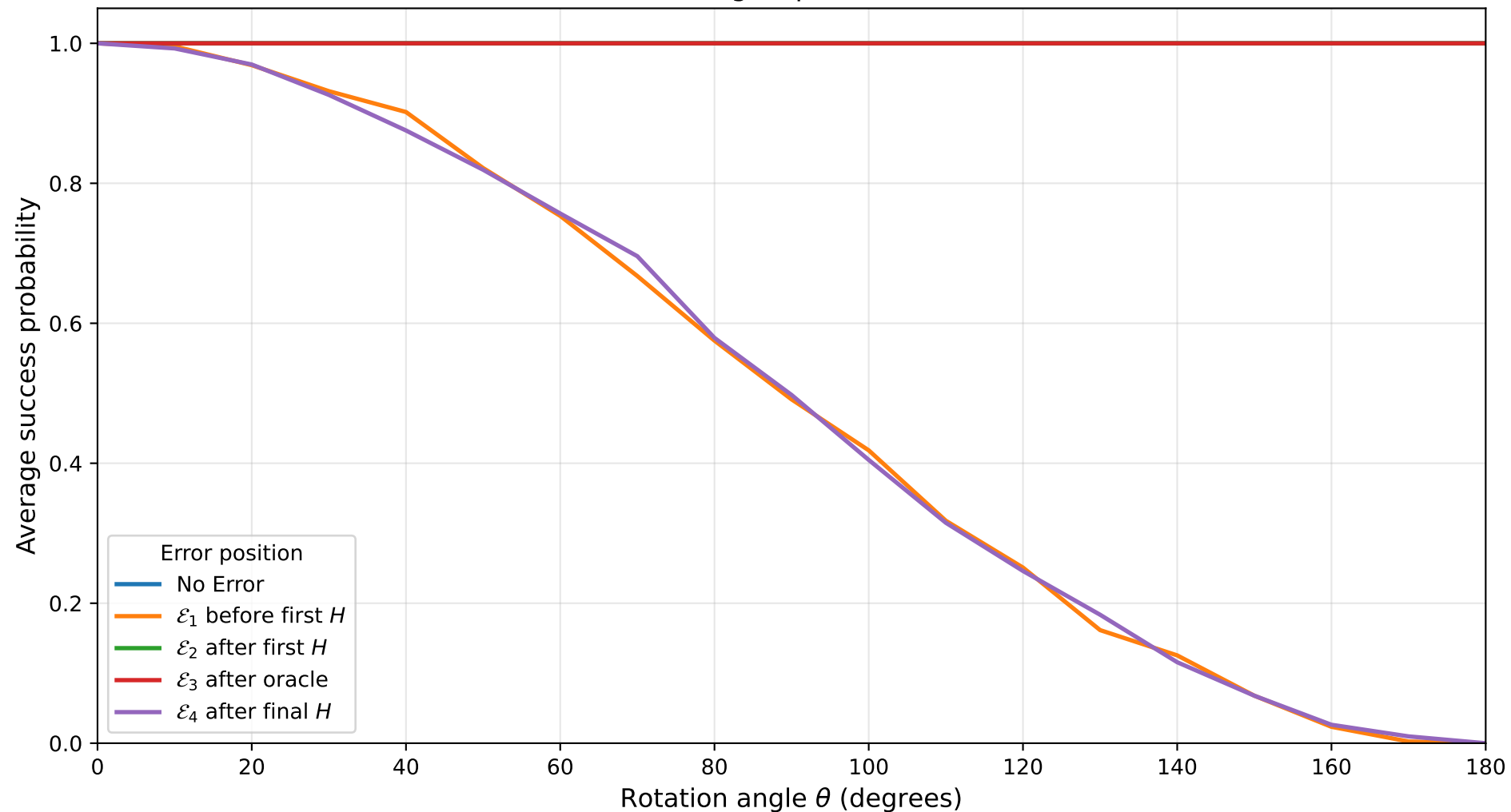
Deutsch-Jozsa Algorithm under Rotation Errors n=9, axis=X, target qubit=8, shots=1024
