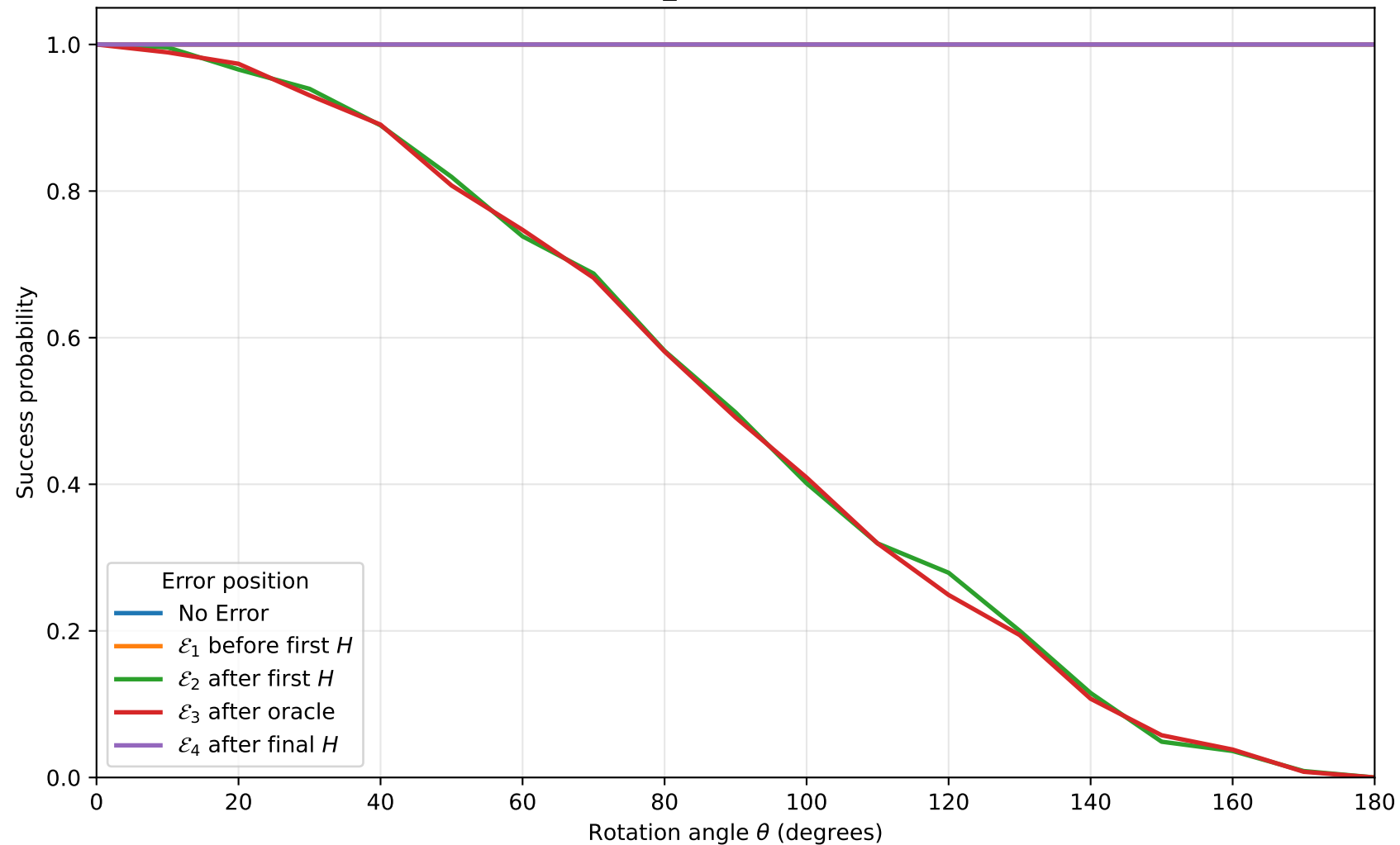
DJA success under rotation errors function=constant_1, n=9, axis=Z, shots=1024
