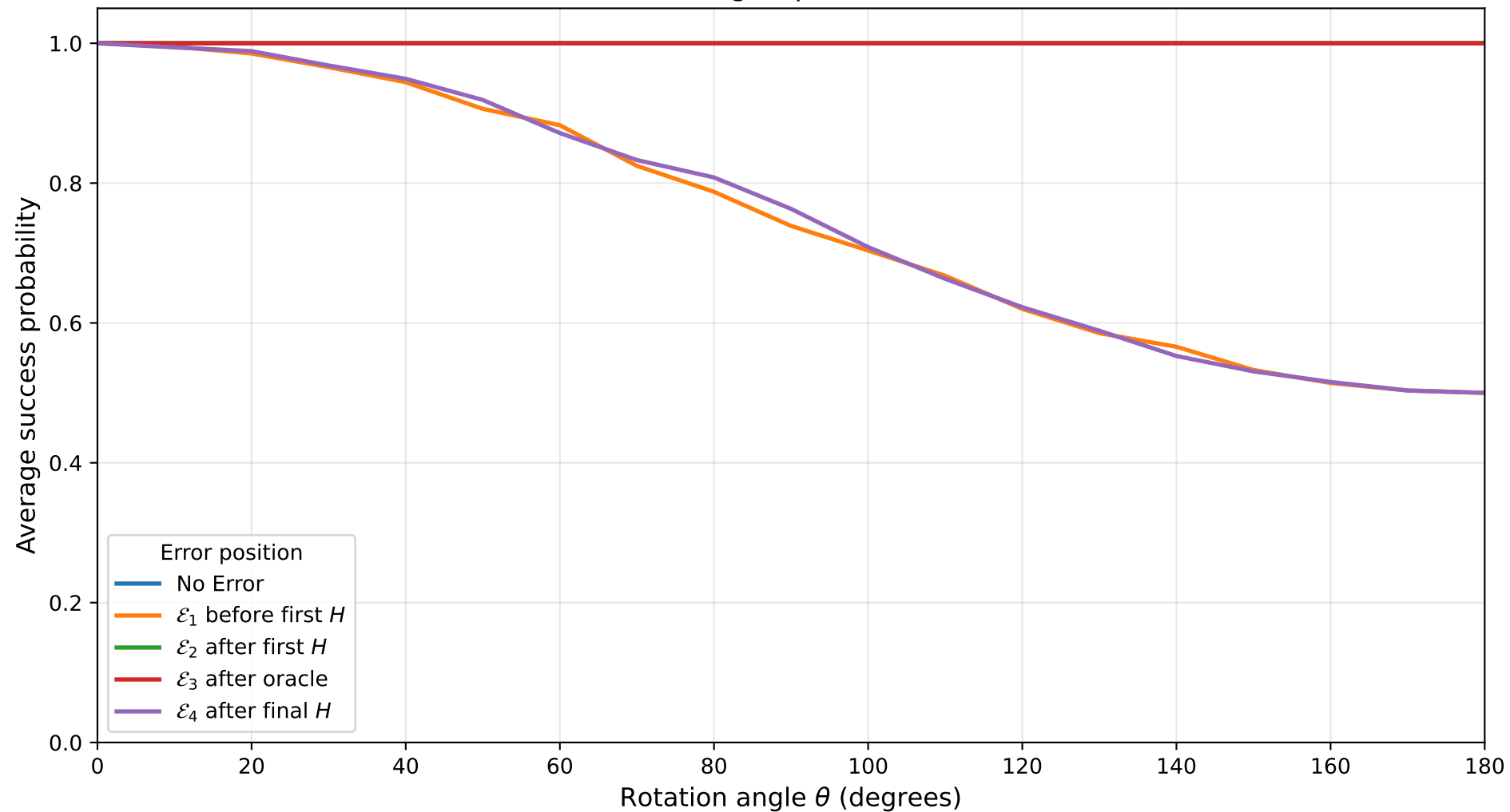
Deutsch-Jozsa Algorithm under Rotation Errors n=9, axis=X, target qubit=7, shots=1024
