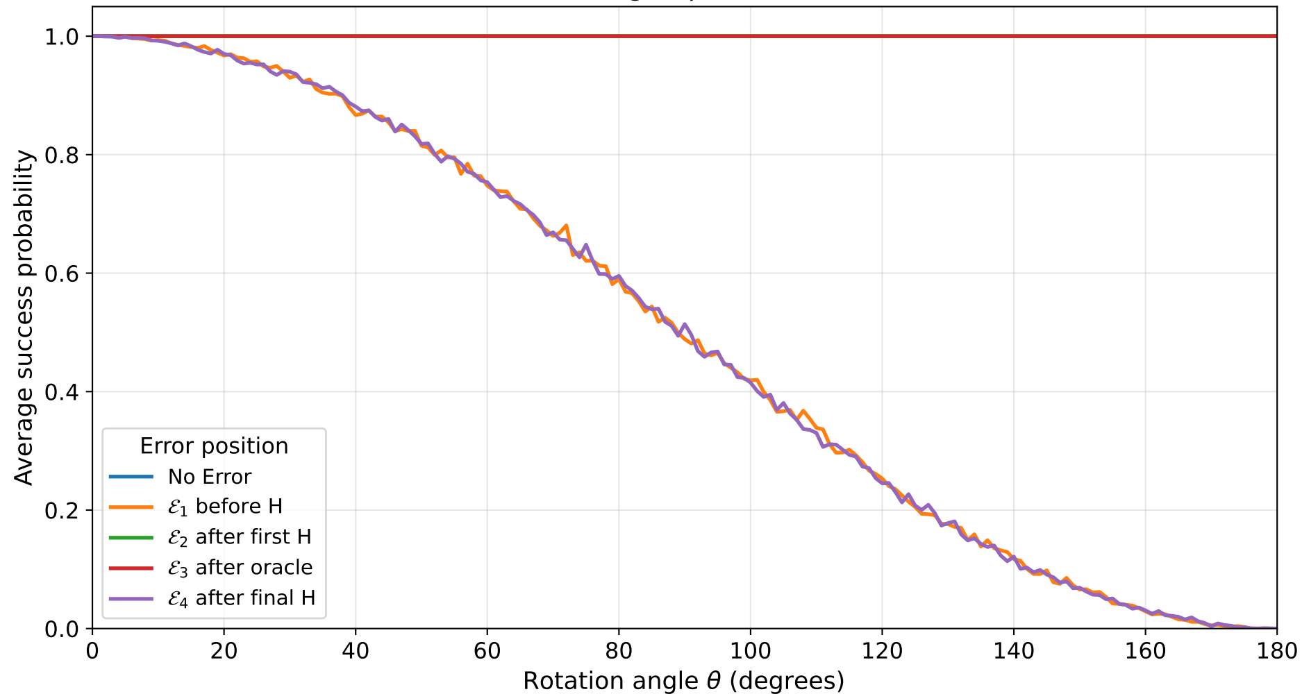
Average Deutsch-Jozsa success under rotation errors n=1, axis=X, target qubit=0, shots=1024
