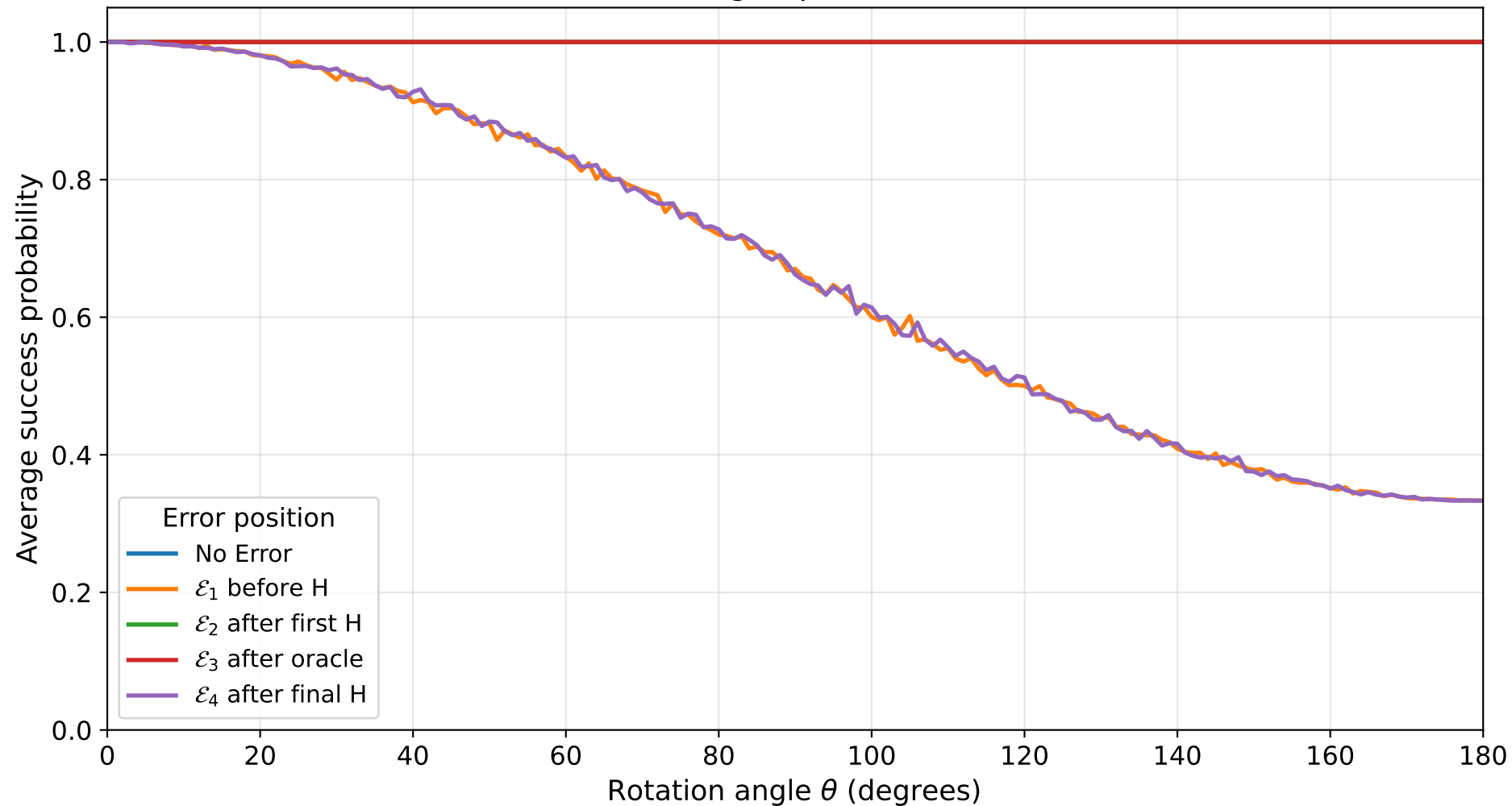
Average Deutsch-Jozsa success under rotation errors n=5, axis=X, target qubit=2, shots=1024
