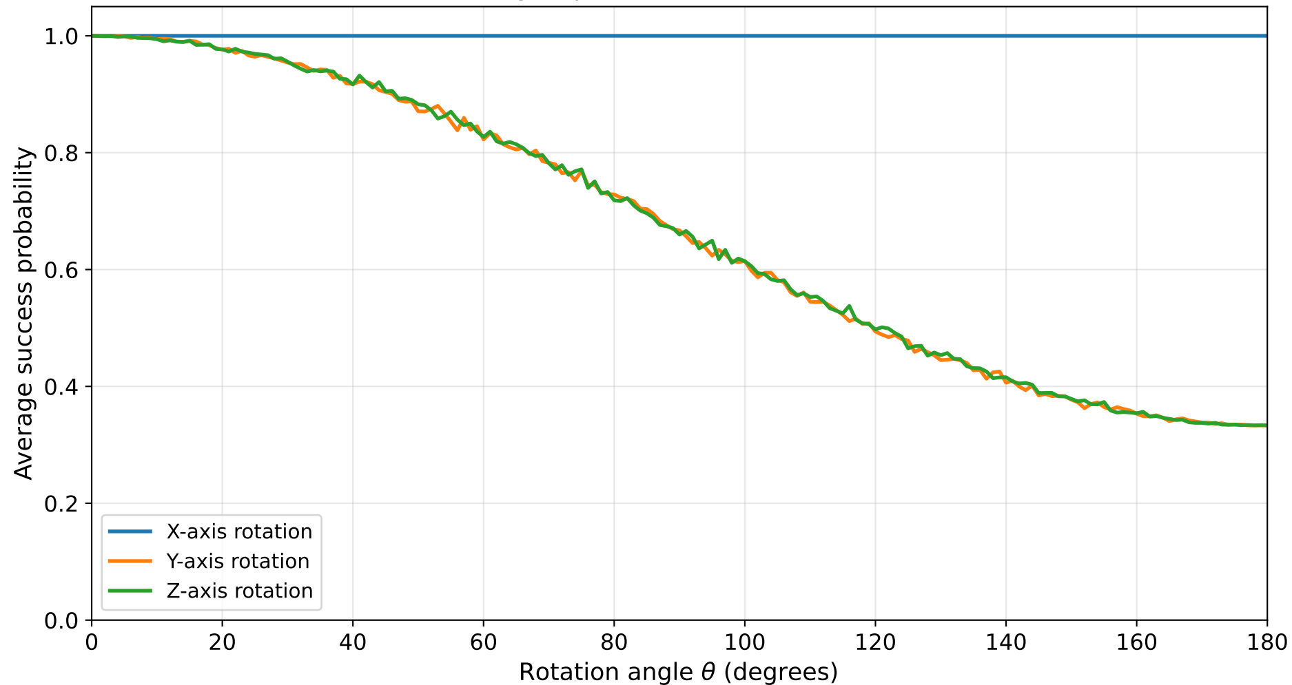
Comparison of rotation axes n=5, target qubit=2, error= \varepsilon_2 after first H
