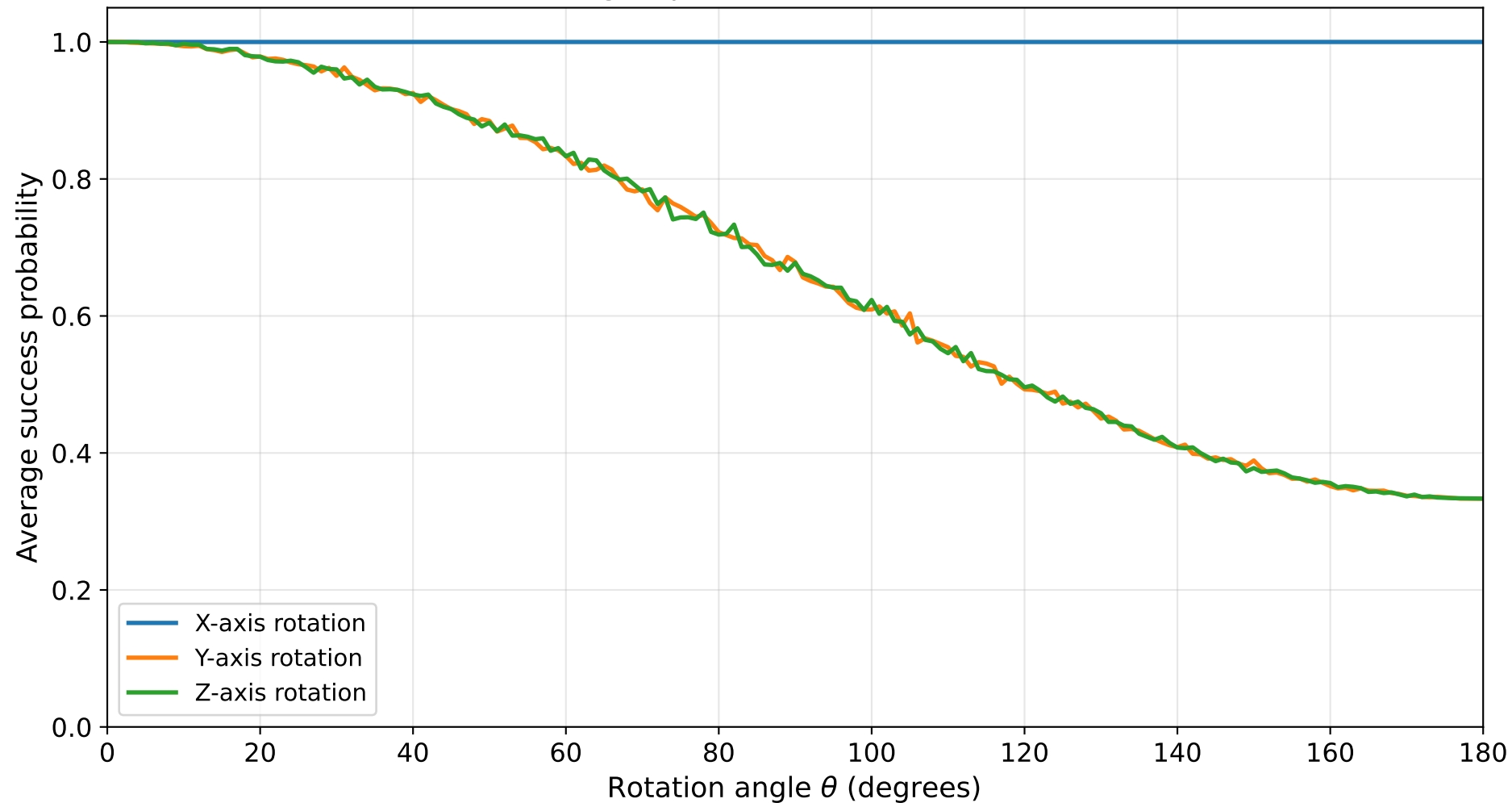
Comparison of rotation axes n=5, target qubit=2, error= \varepsilon_3 after oracle
