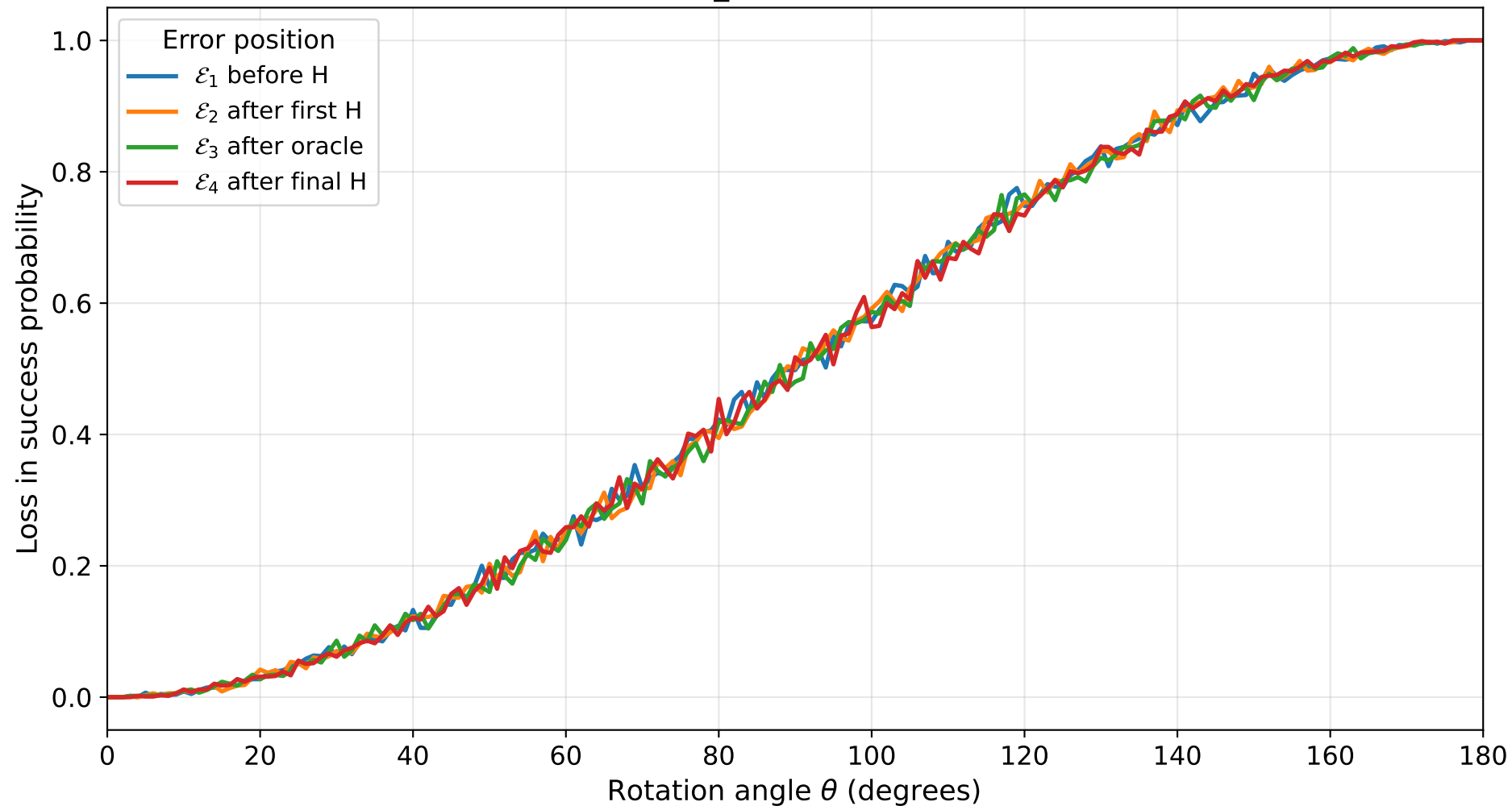
Error impact on Deutsch-Jozsa success function=constant_1, n=5, axis=Y, shots=1024
