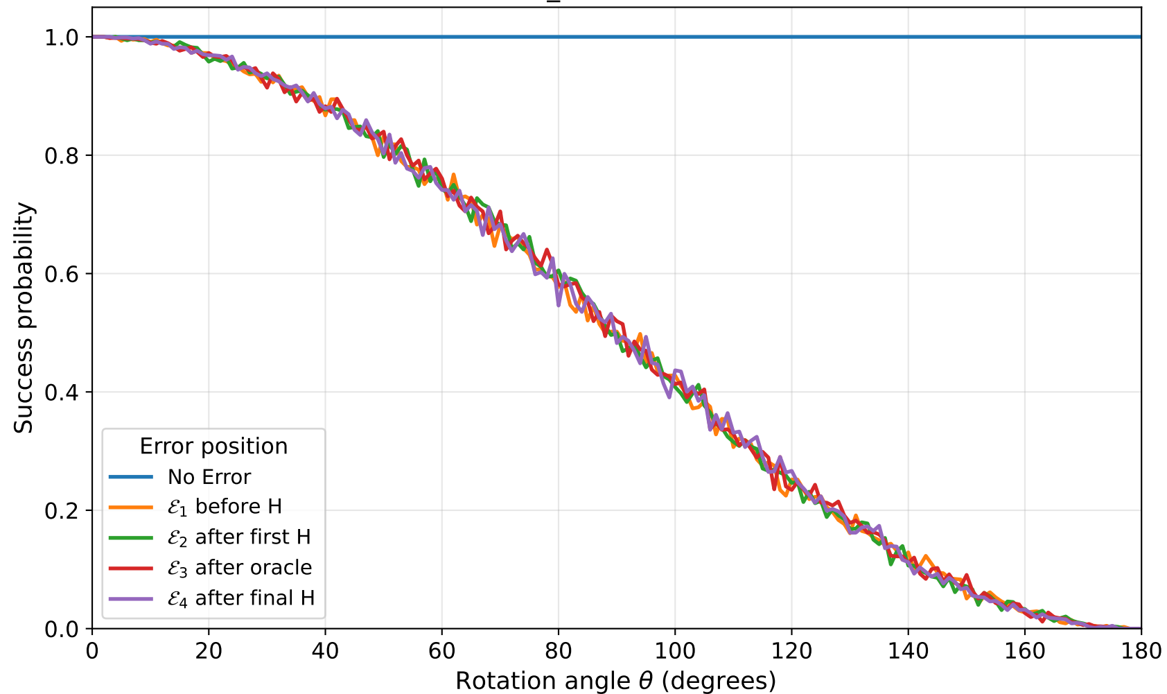
Deutsch-Jozsa success under rotation errors function=constant_1, n=5, axis=Y, shots=1024
