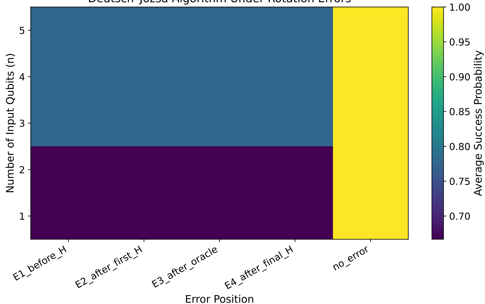
Average Success Probability Deutsch-Jozsa Algorithm Under Rotation Errors
