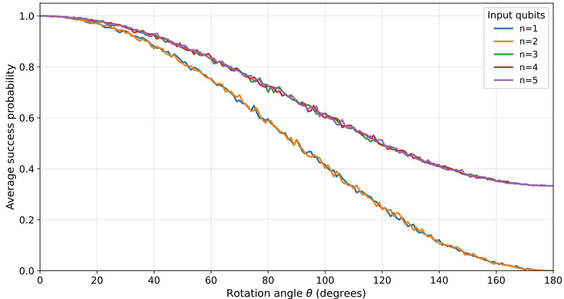
Scaling with number of qubits axis=X, error= \mathcal{E}_4 after final H
