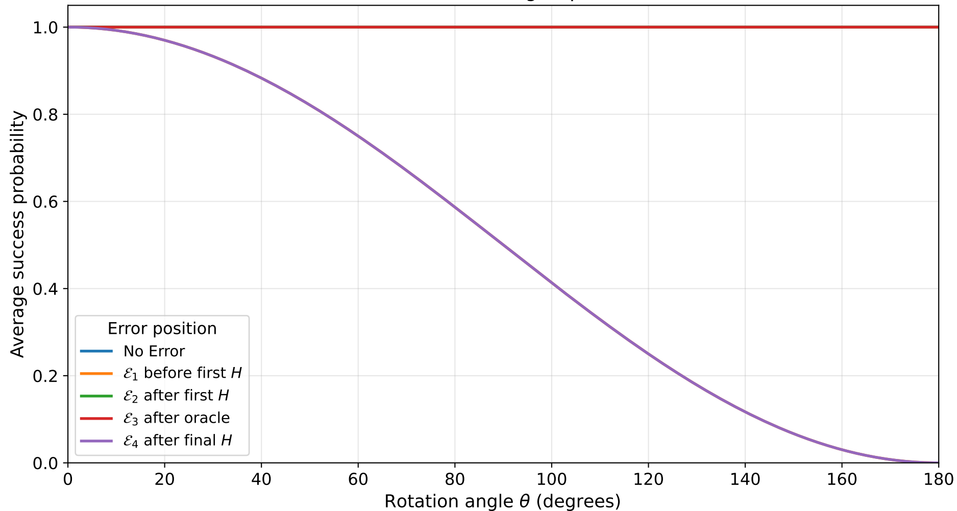
Average Deutsch-Jozsa success under rotation errors n=1, axis=X, target qubit=0
