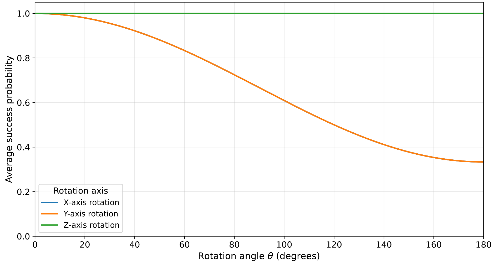
Comparison of rotation axes n=5, target qubit=2, error= \varepsilon_1 before first H
