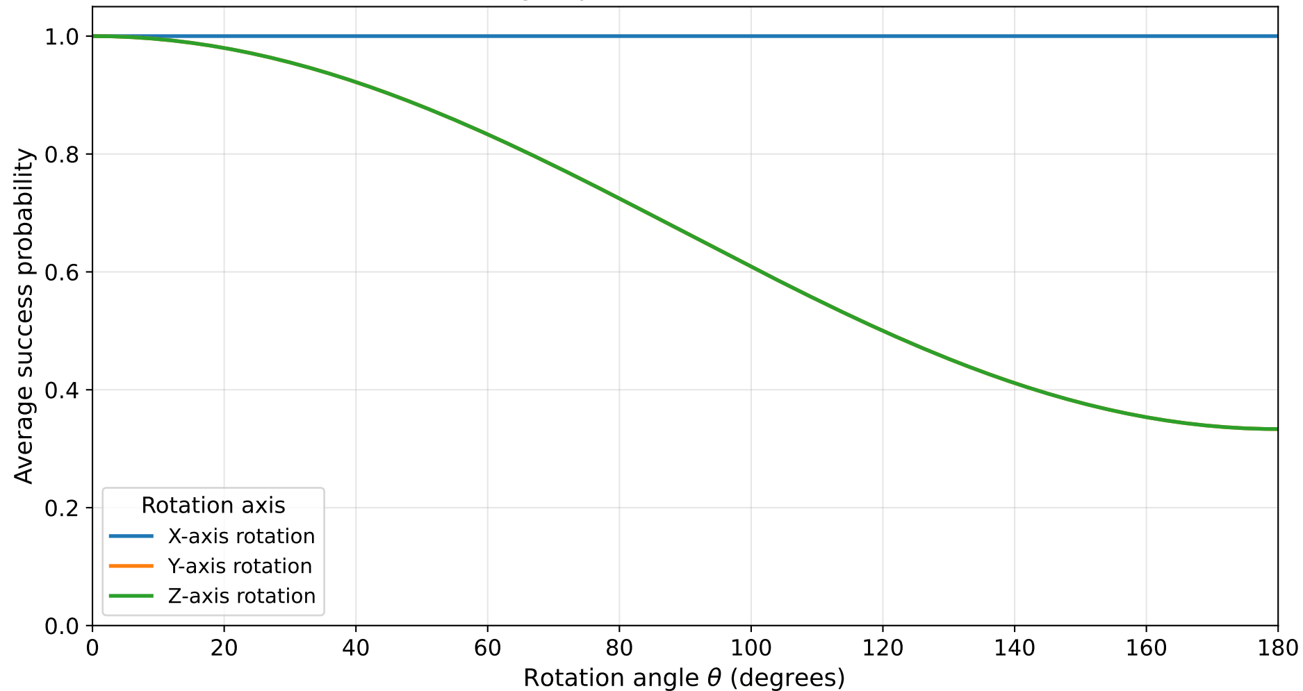
Comparison of rotation axes n=5, target qubit=2, error= \mathcal{E}_2 after first H
