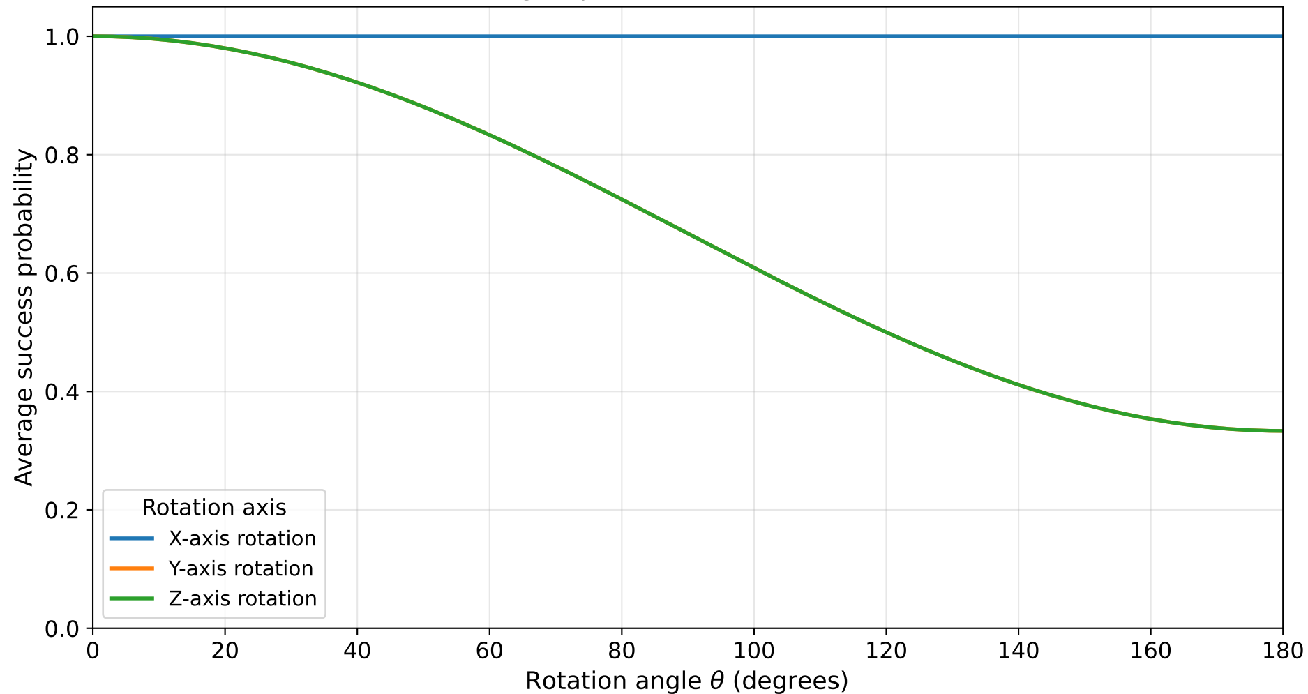
Comparison of rotation axes n=5, target qubit=2, error= \mathcal{E}_3 after oracle
