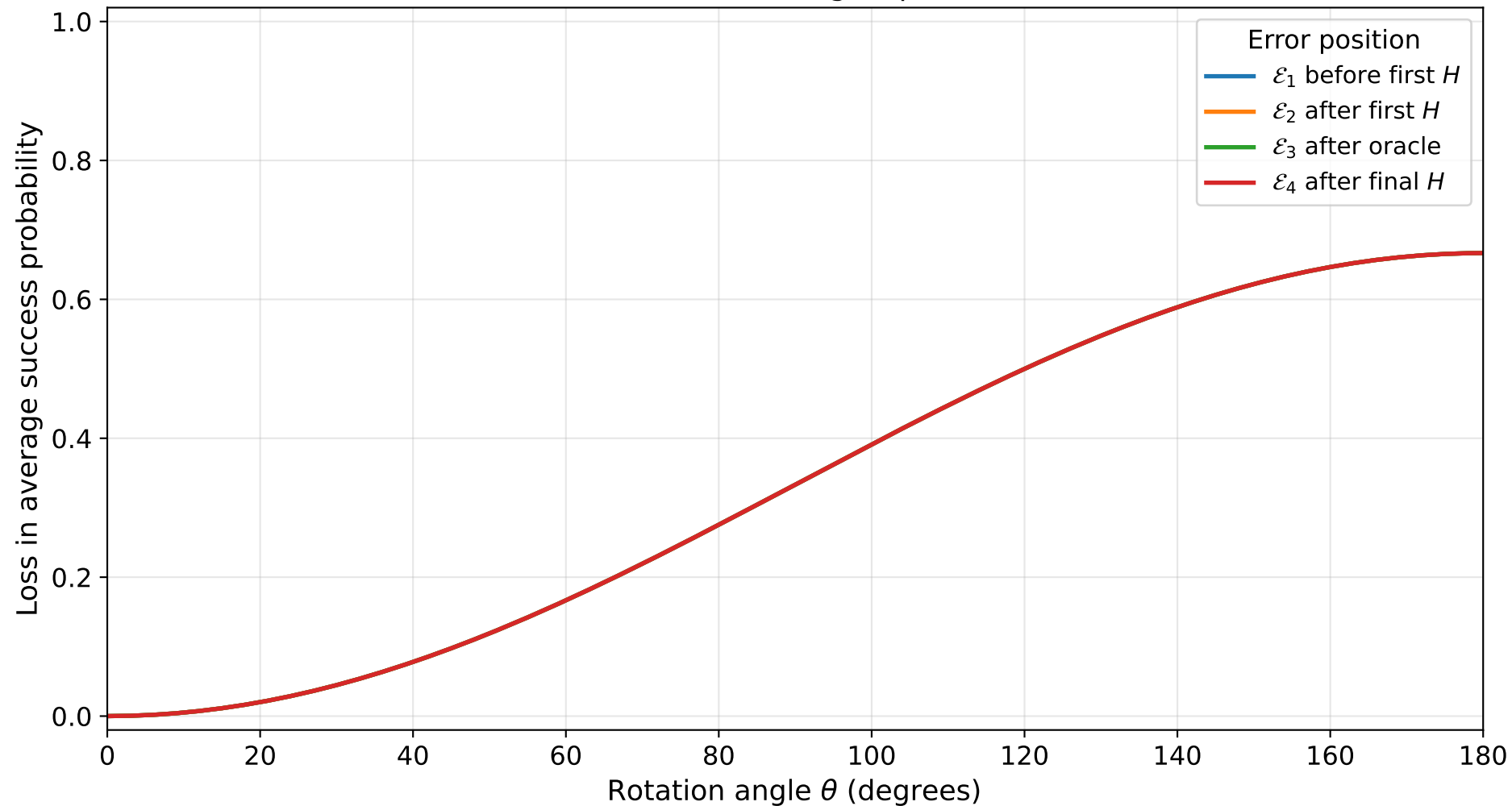
Error impact on Deutsch-Jozsa success n=5, axis=Y, target qubit=2
