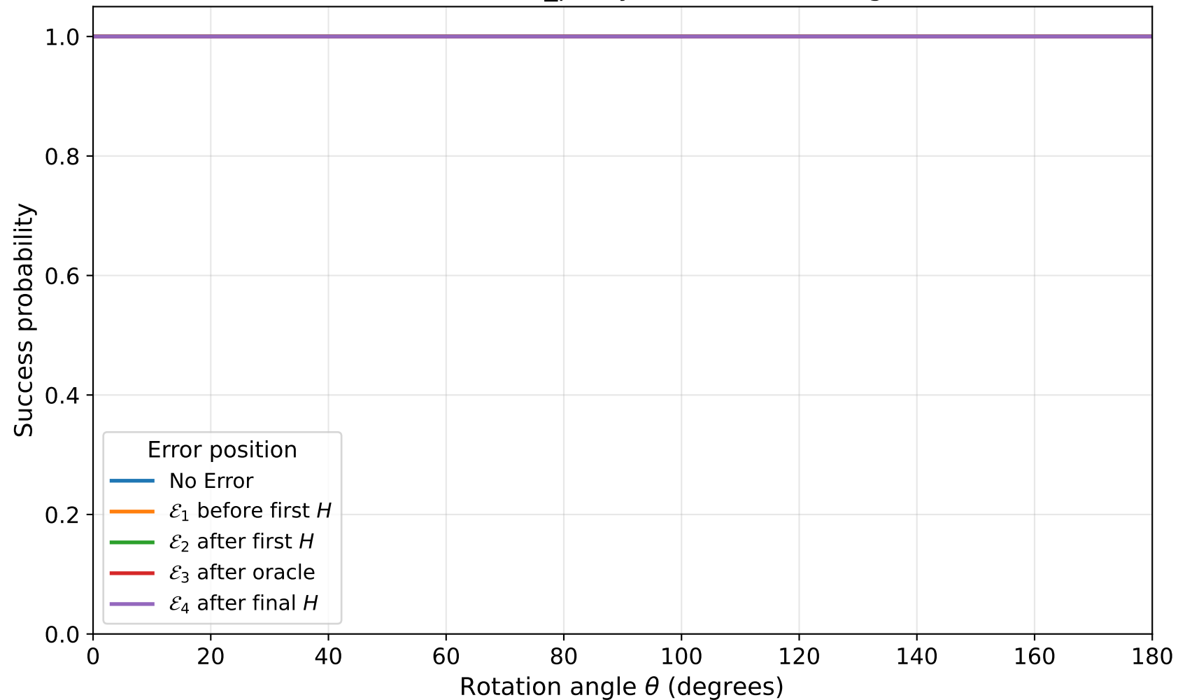
Deutsch-Jozsa success under rotation errors function=balanced_parity, n=5, axis=X, target=2
