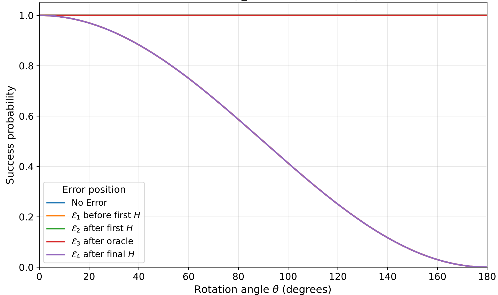
Deutsch-Jozsa success under rotation errors function=constant_1, n=5, axis=X, target=2
