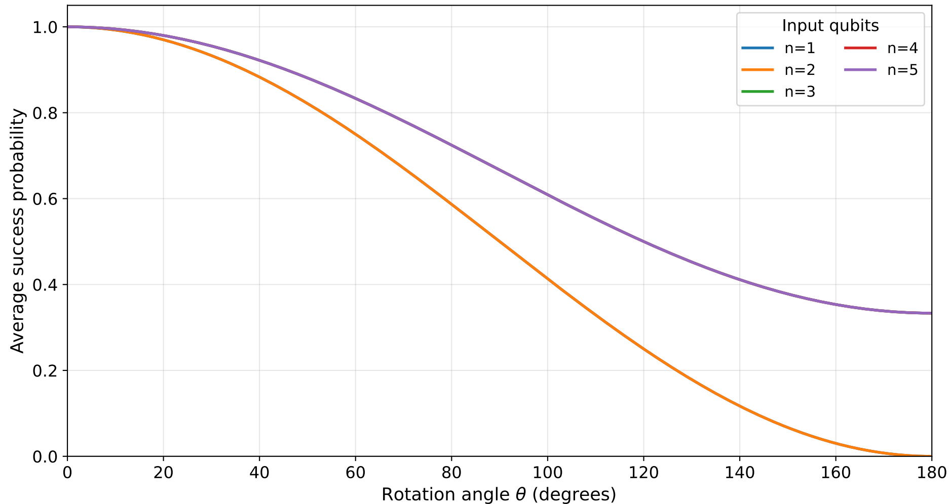
Scaling with number of input qubits axis=Y, error= \mathcal{E}_1 before first H
