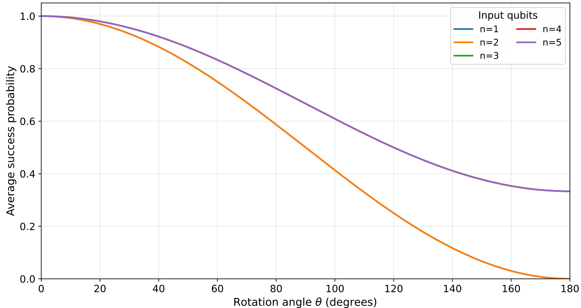
Scaling with number of input qubits axis=Y, error= \mathcal{E}_4 after final H
