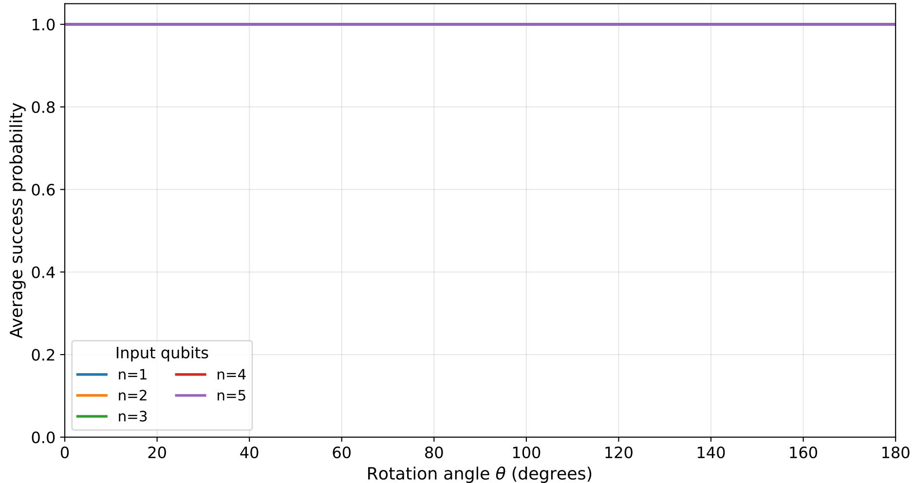
Scaling with number of input qubits axis=Z, error= \varepsilon_1 before first H
