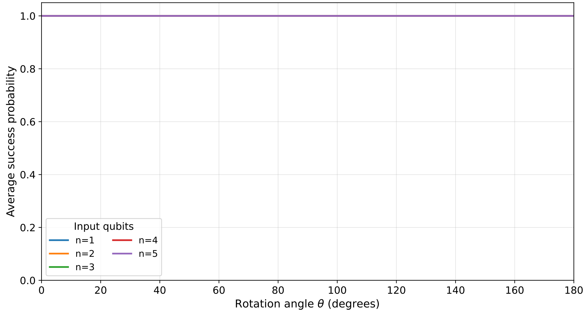
Scaling with number of input qubits axis=Z, error= \mathcal{E}_4 after final H
