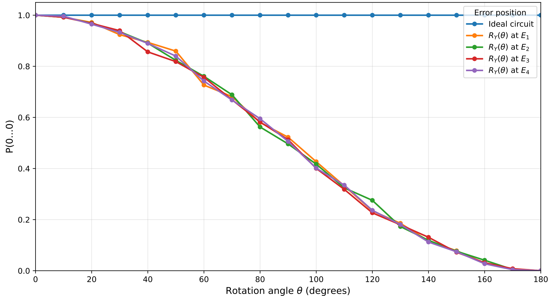
Probability under Y-Axis Rotation Errors Constant 1, n=9 , target qubit=4, shots=1024
