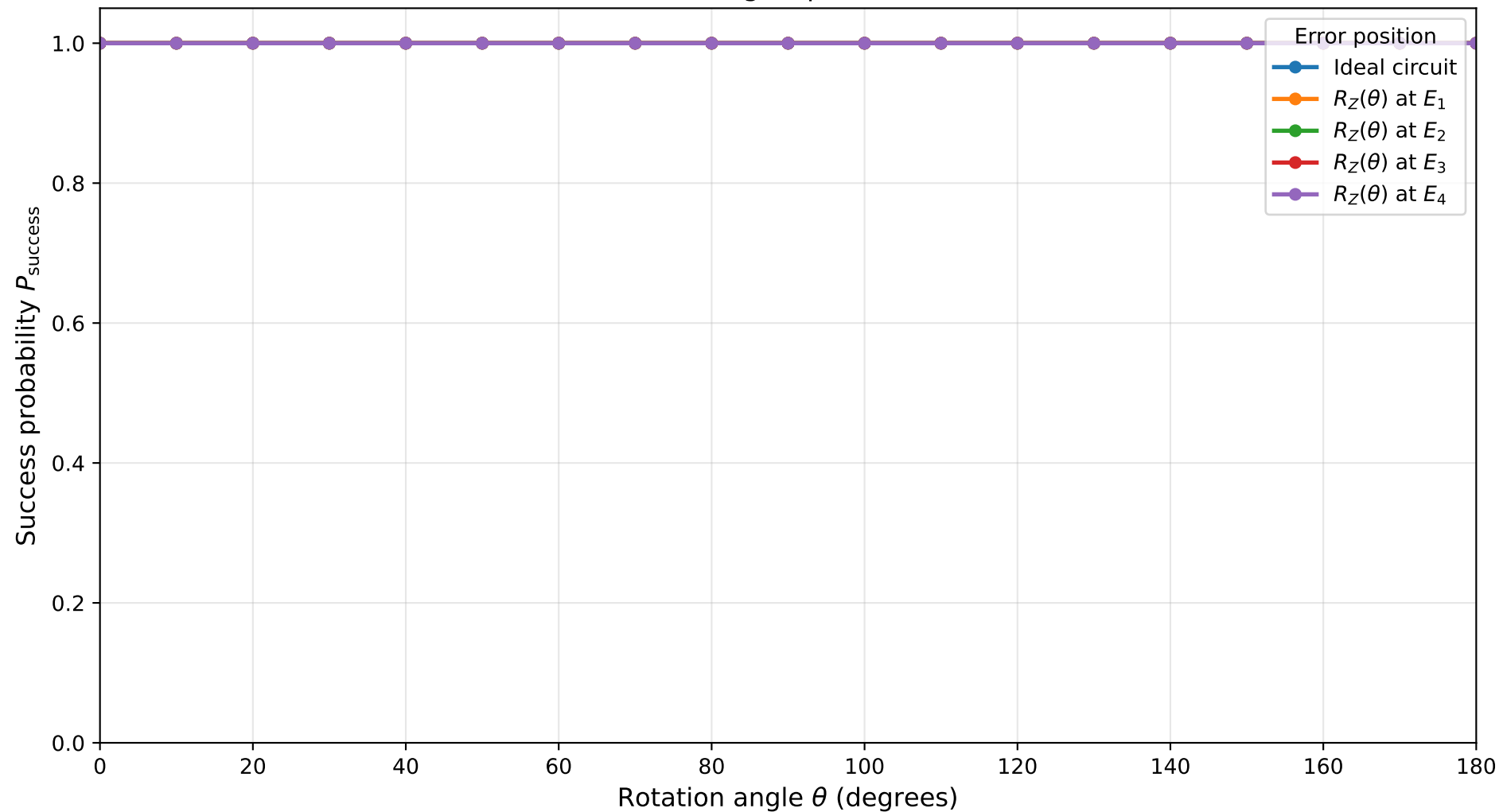
Success Probability under Z-Axis Rotation Errors Balanced, n=9, target qubit=4, shots=1024
