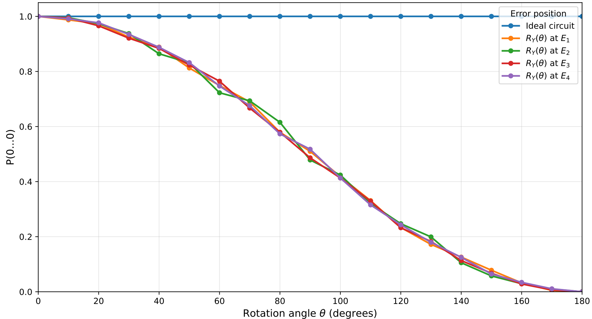
Probability under Y-Axis Rotation Errors Constant 0, n=9 , target qubit=4, shots=1024
