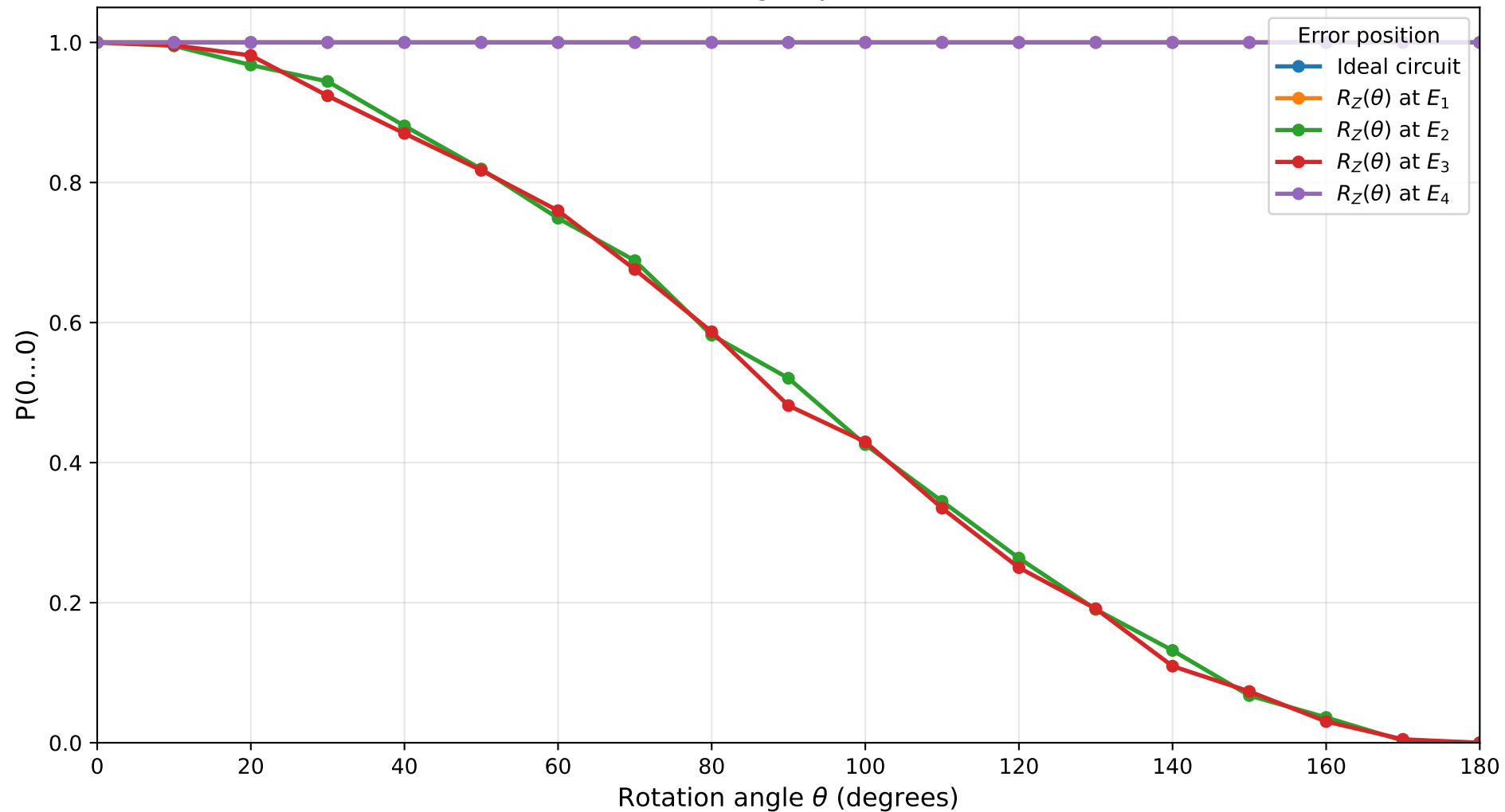
Probability under Z-Axis Rotation Errors Constant 0, n=9 , target qubit=4, shots=1024
