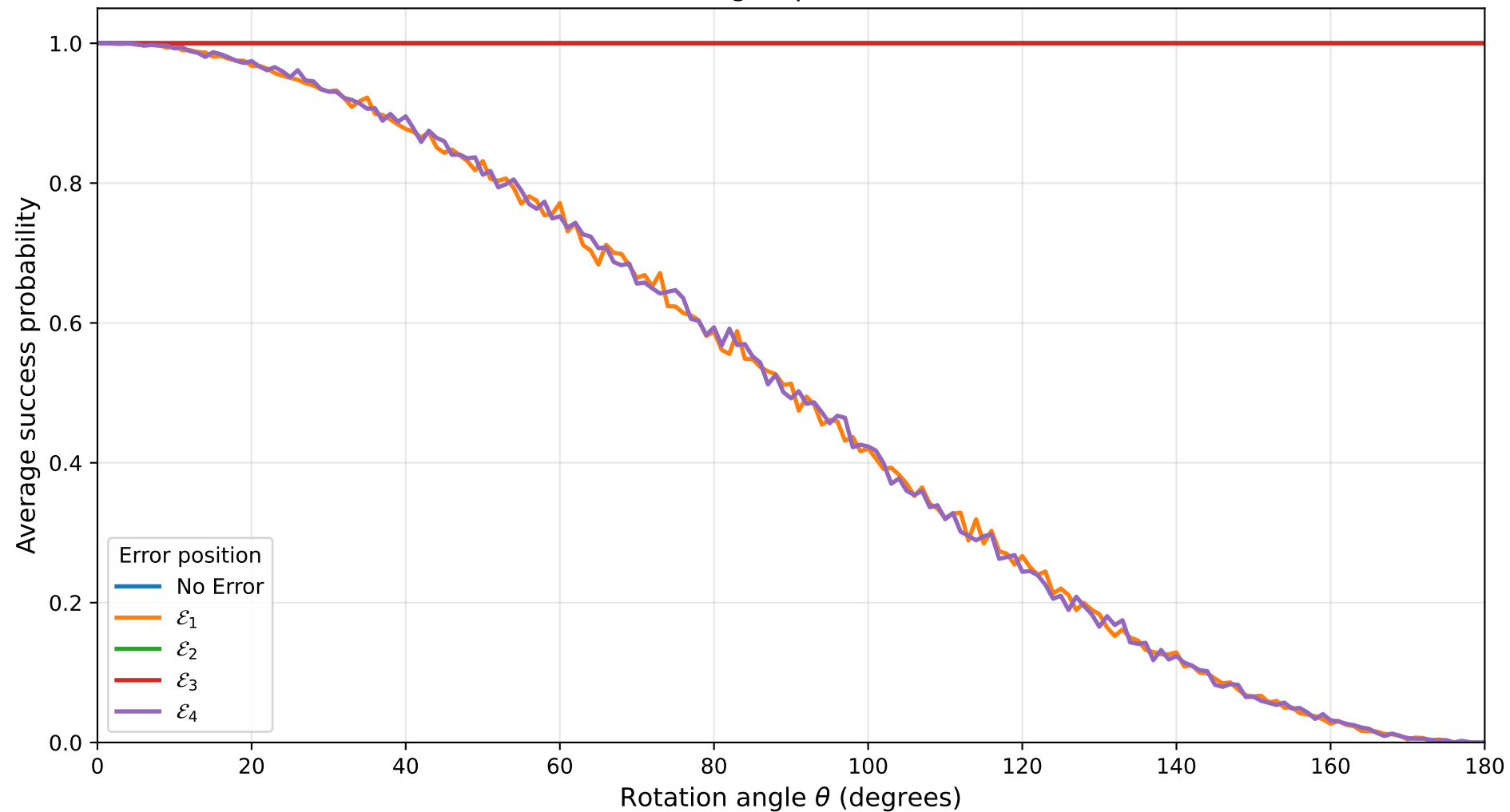
Deutsch-Jozsa Algorithm under Rotation Errors n=6, axis=X, target qubit=5, shots=1024
