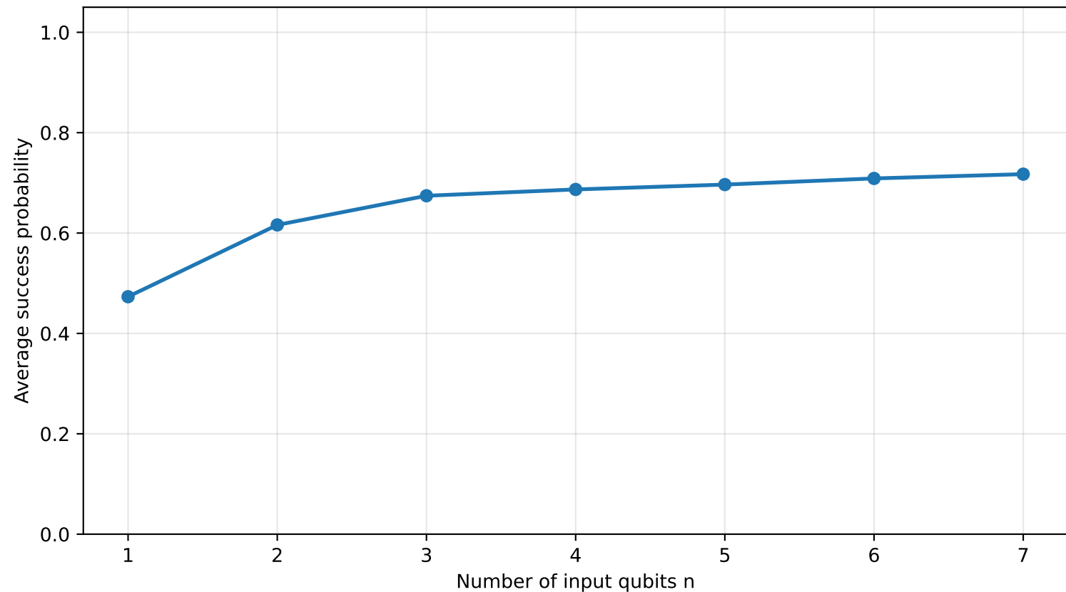
Scalability under \mathcal{E}_4 noise axis=X, \theta=90^\circ , shots=1024
