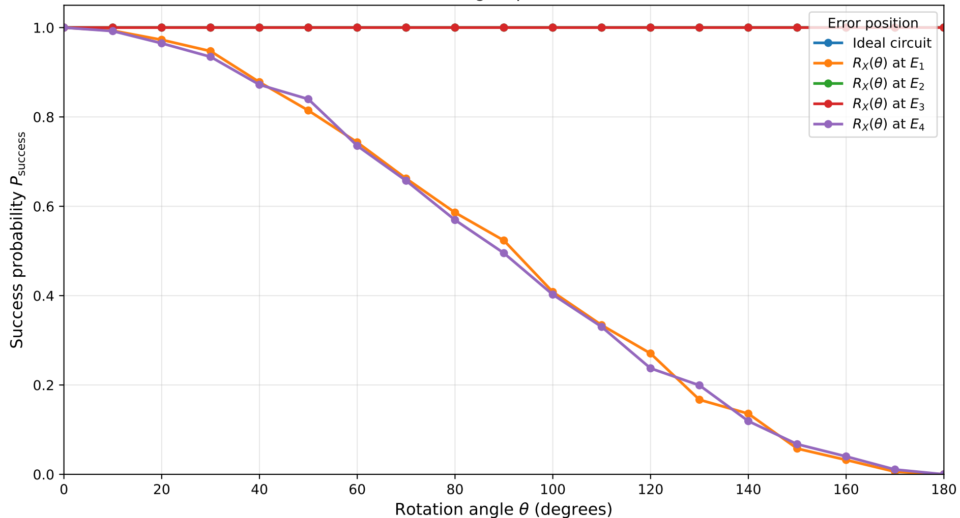
Success Probability under X-Axis Rotation Errors Balanced, n=5 , target qubit=4, shots=1024
