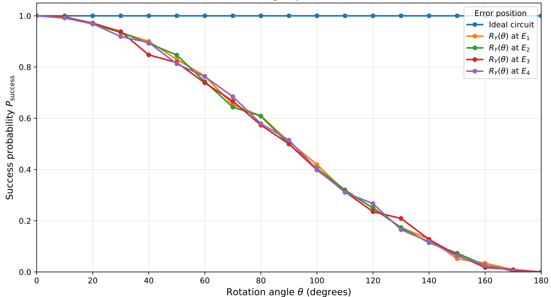
Success Probability under Y-Axis Rotation Errors Balanced, n=5 , target qubit=4, shots=1024
