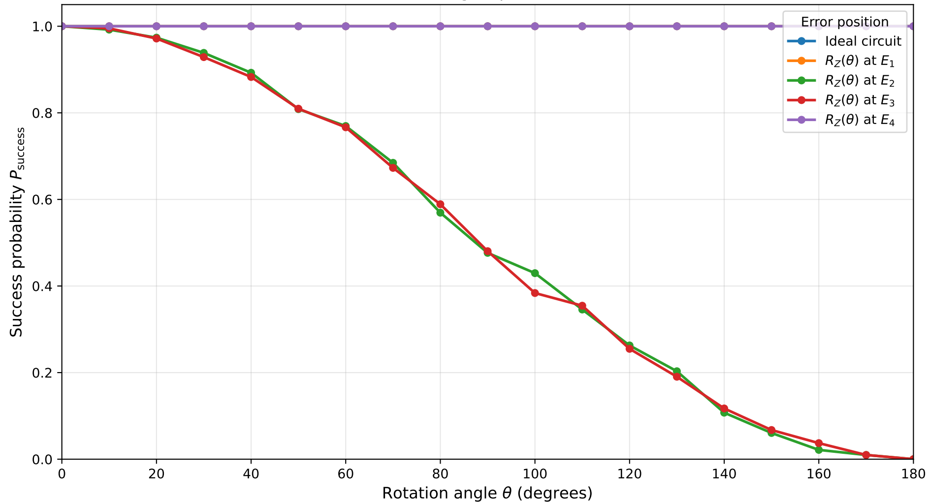
Success Probability under Z-Axis Rotation Errors Balanced, n=5 , target qubit=4, shots=1024
