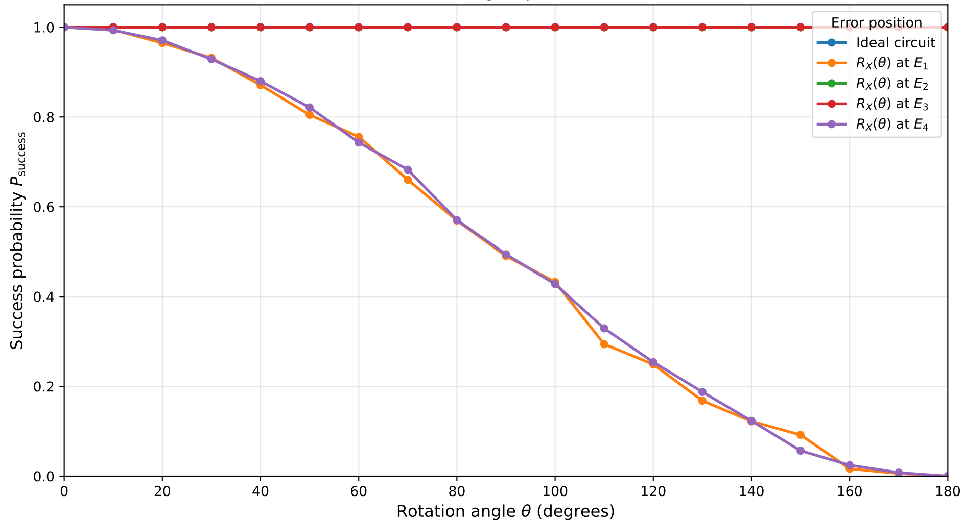
Success Probability under X-Axis Rotation Errors Constant 0, n=5 , target qubit=4, shots=1024
