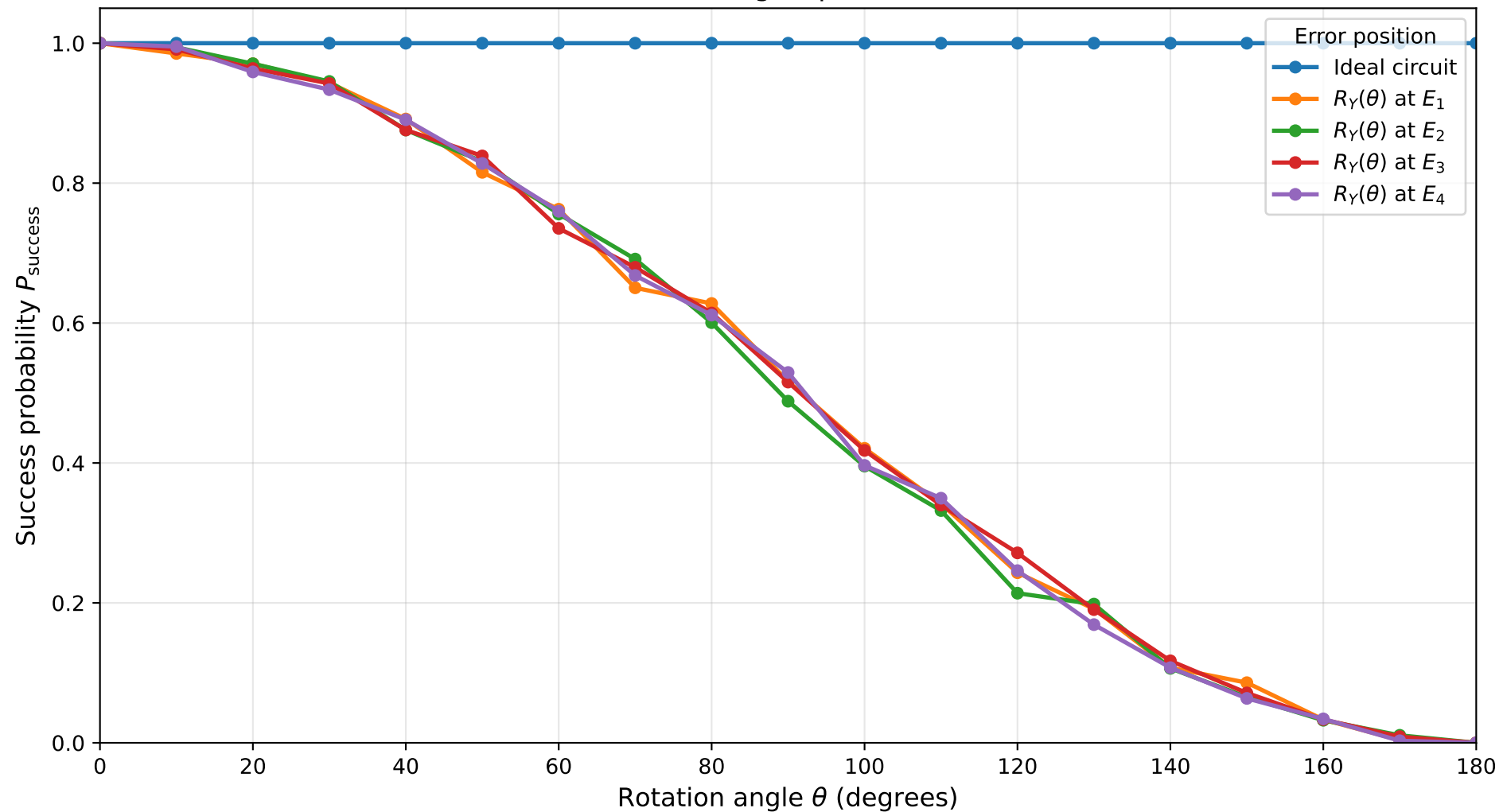
Success Probability under Y-Axis Rotation Errors Constant 0, n=5 , target qubit=4, shots=1024
