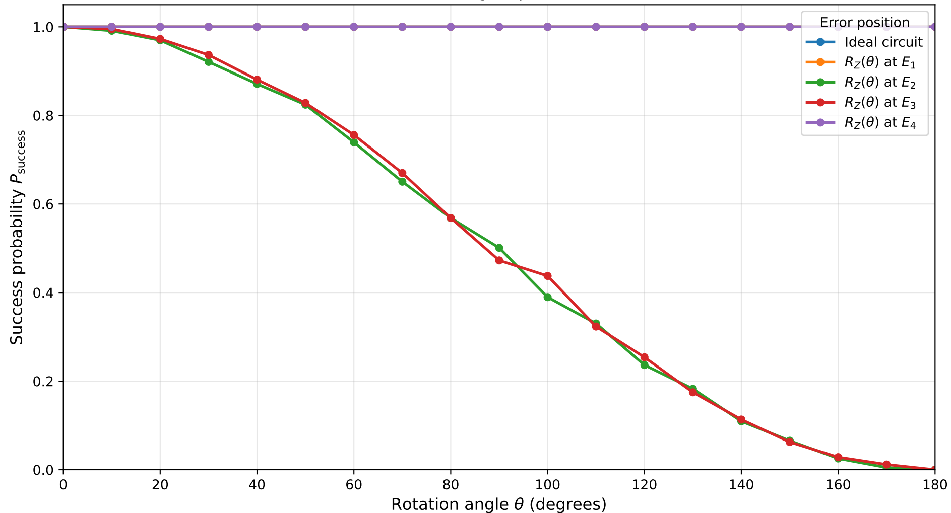
Success Probability under Z-Axis Rotation Errors Constant 0, n=5 , target qubit=4, shots=1024
