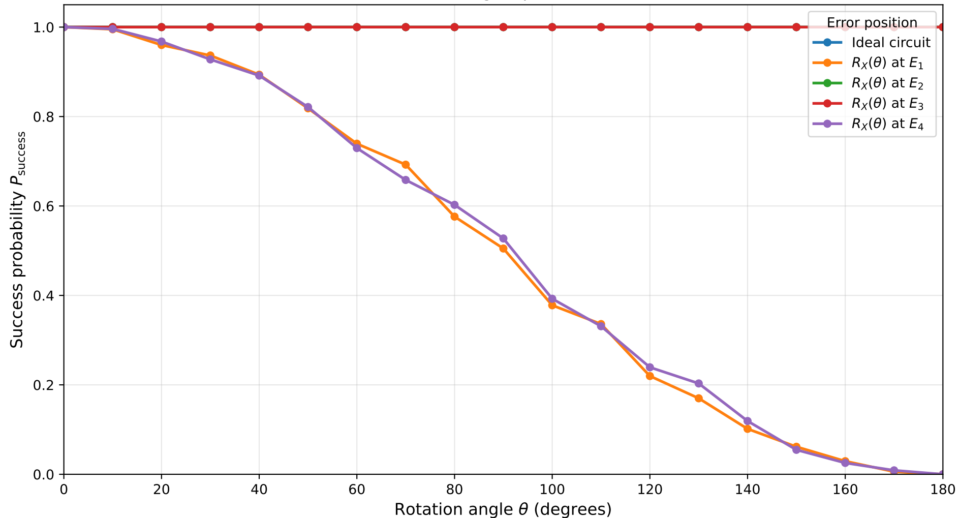
Success Probability under X-Axis Rotation Errors Constant 1, n=5 , target qubit=4, shots=1024
