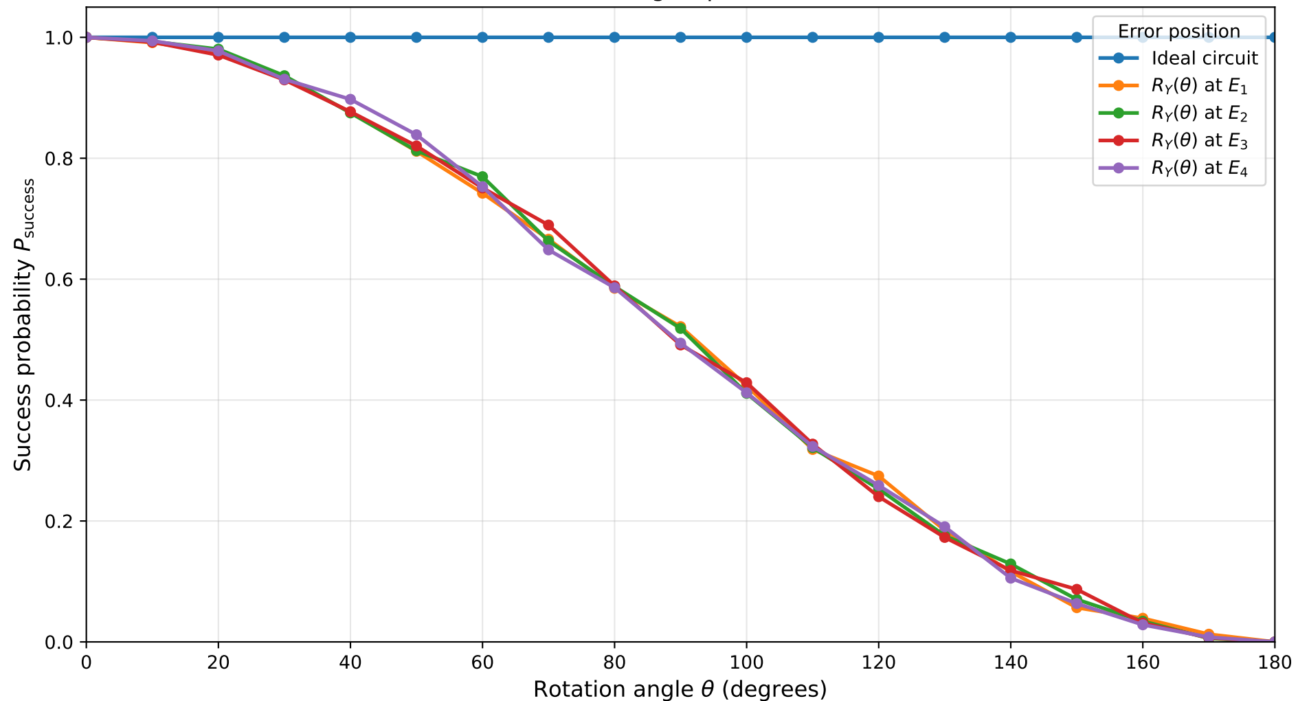
Success Probability under Y-Axis Rotation Errors Constant 1, n=5 , target qubit=4, shots=1024
