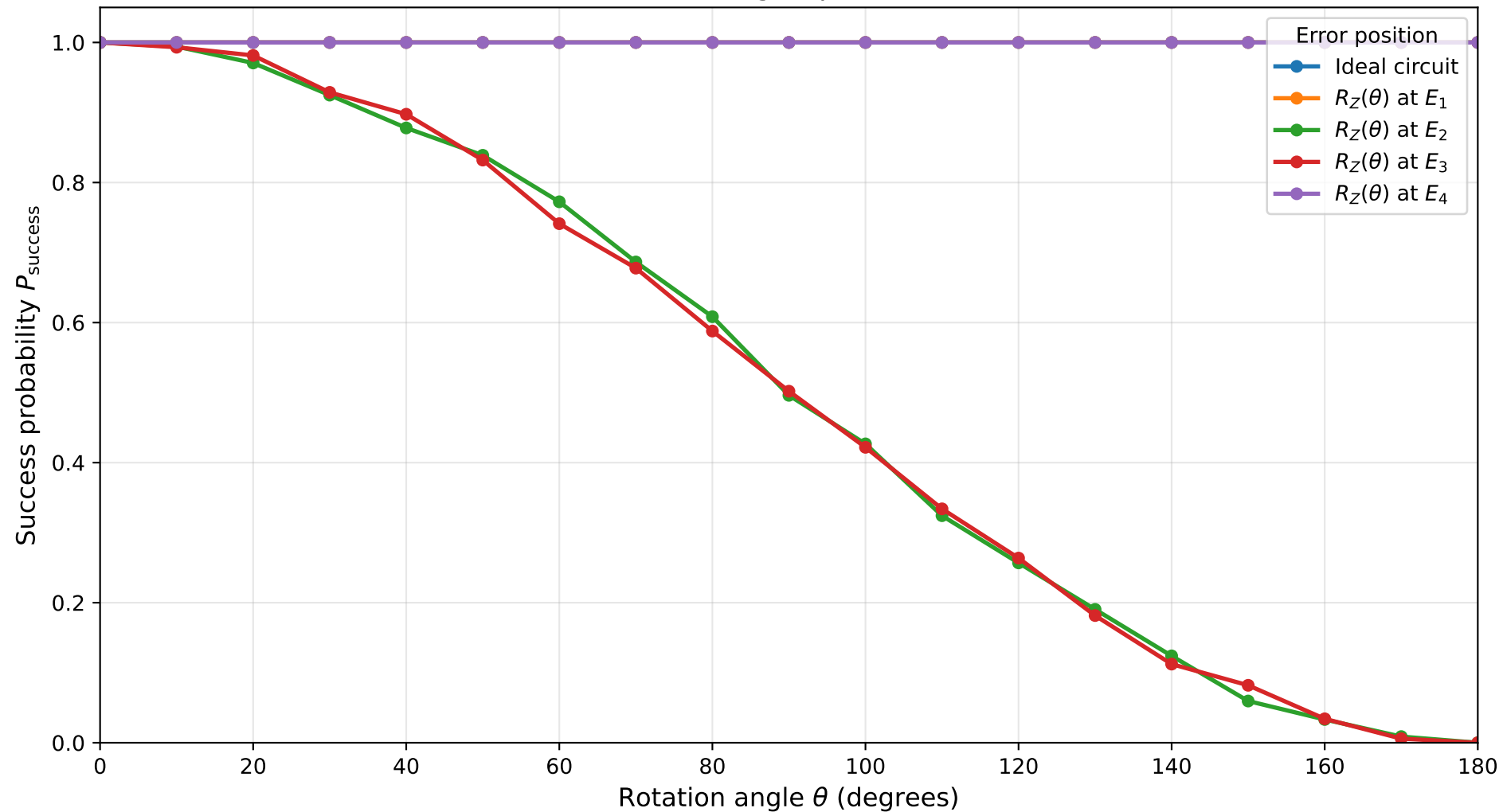
Success Probability under Z-Axis Rotation Errors Constant 1, n=5 , target qubit=4, shots=1024
