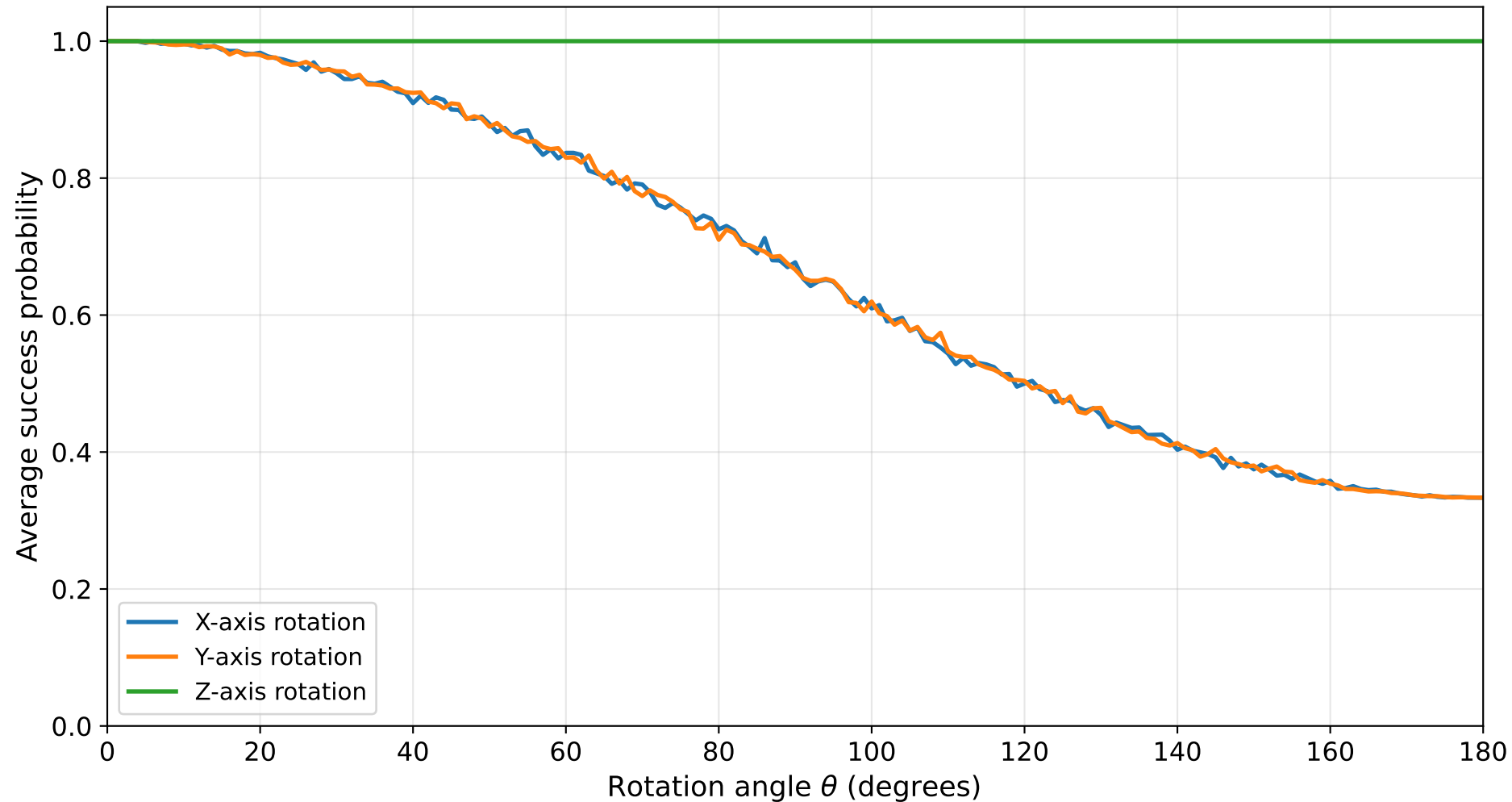
Comparison of rotation axes n=5, target qubit=2, error= \varepsilon_1 before H
