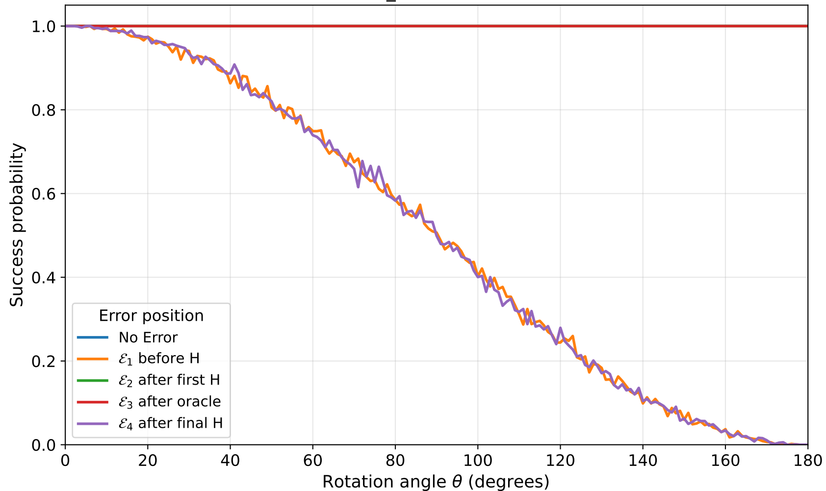
Deutsch-Jozsa success under rotation errors function=constant_1, n=5, axis=X, shots=1024
