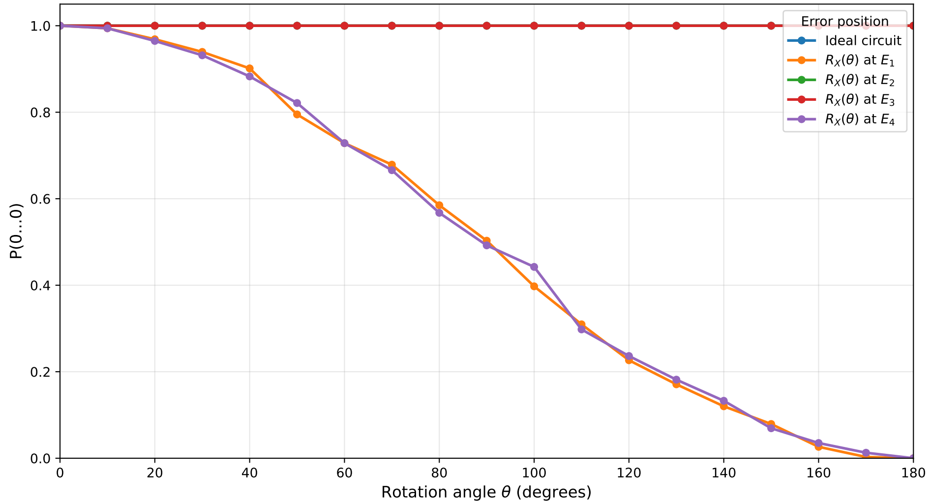
Probability under X-Axis Rotation Errors Constant 0, n=9 , target qubit=1, shots=1024
