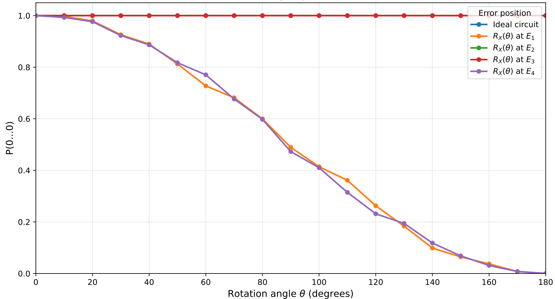
Probability under X-Axis Rotation Errors Constant 0, n=9 , target qubit=4, shots=1024
