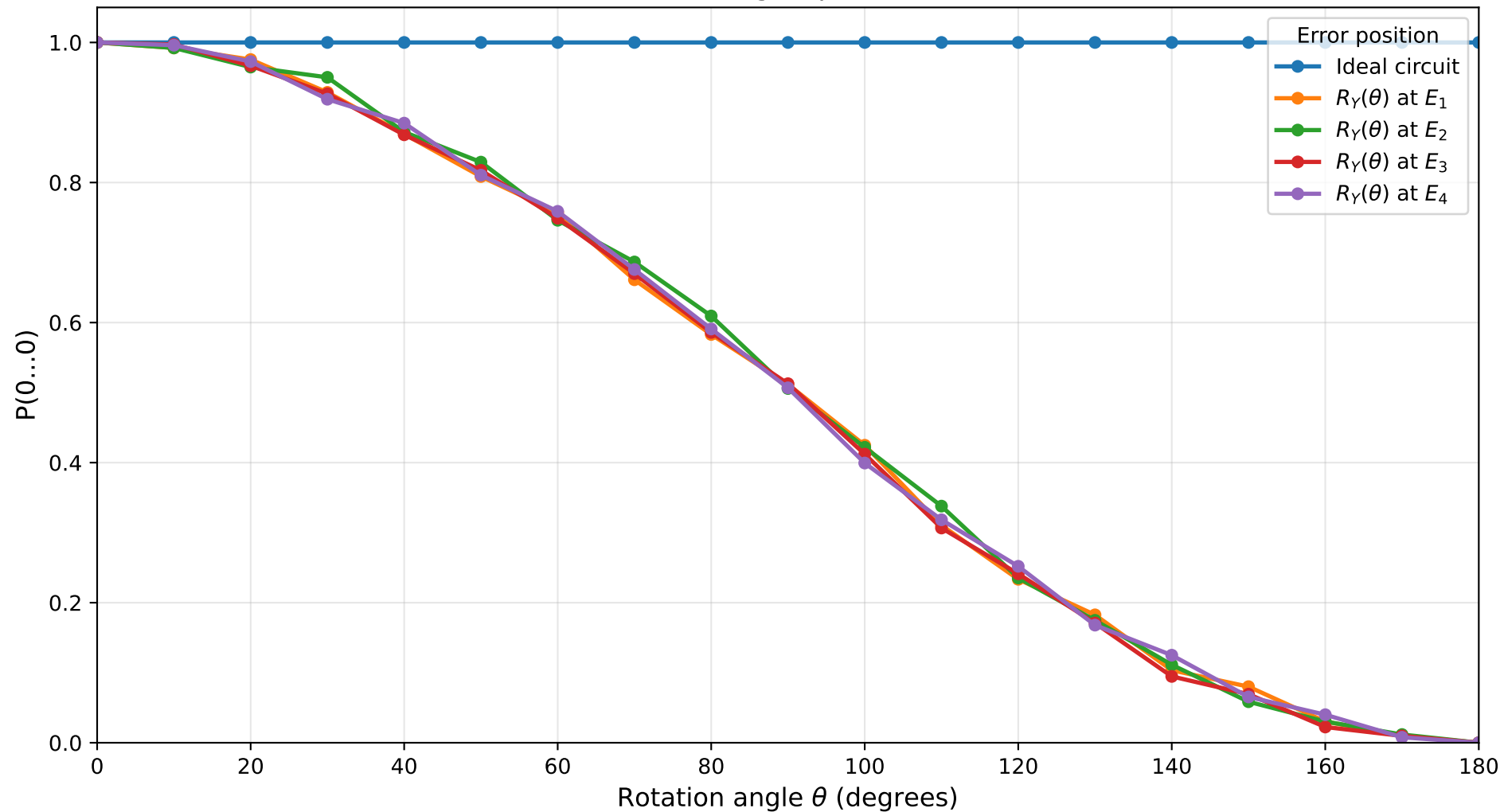
Probability under Y-Axis Rotation Errors Constant 0, n=9 , target qubit=1, shots=1024
