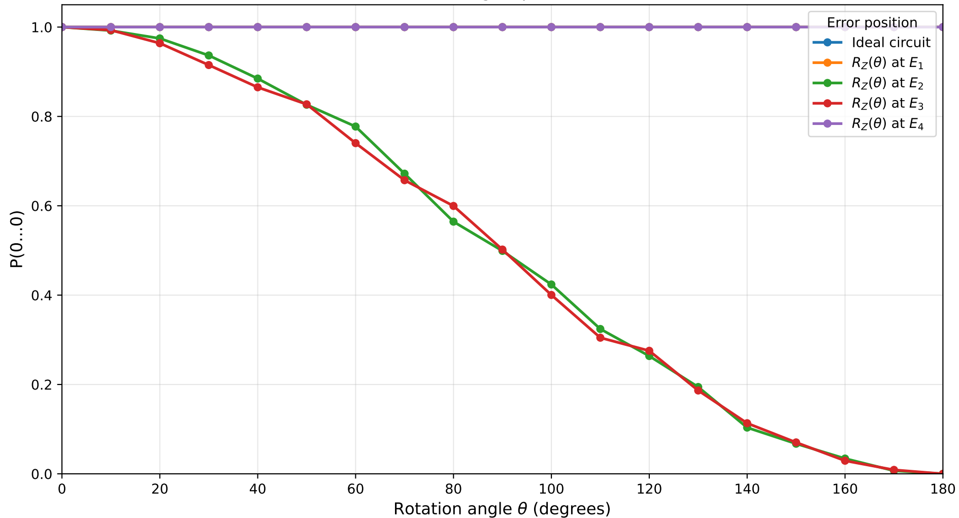
Probability under Z-Axis Rotation Errors Constant 0, n=9 , target qubit=1, shots=1024
