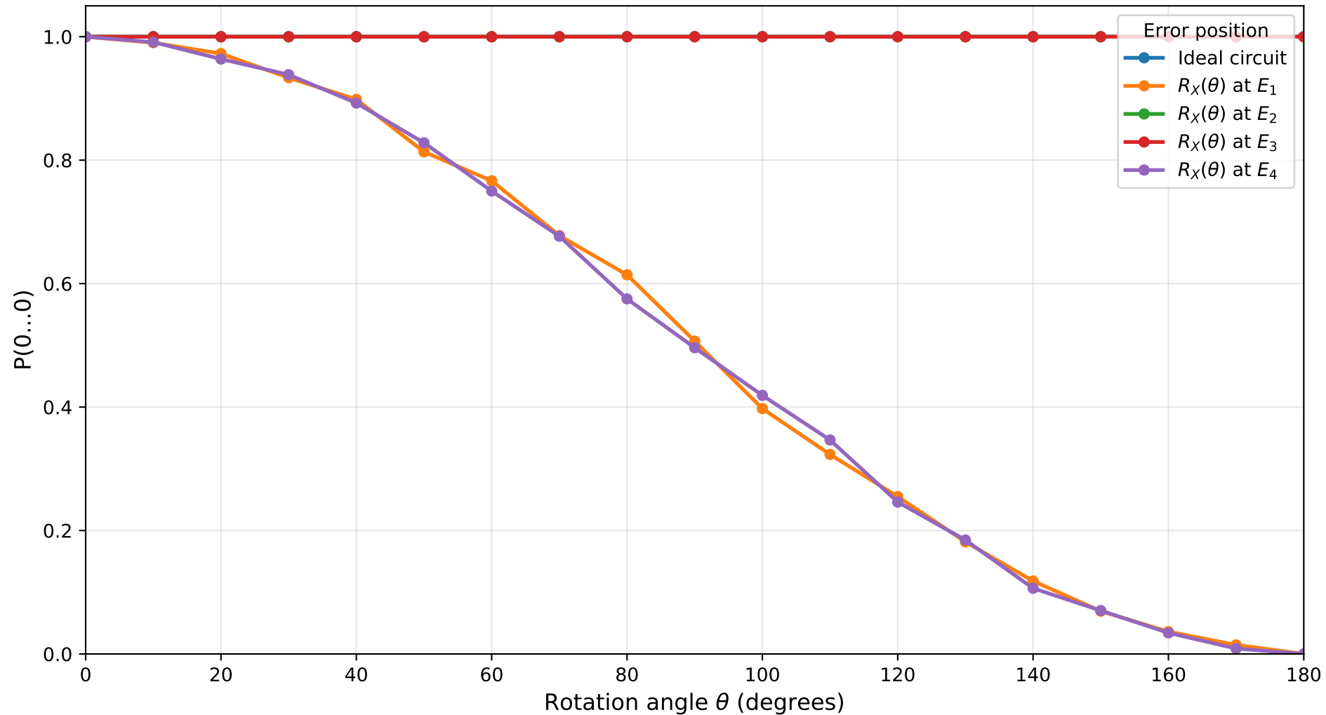
Probability under X-Axis Rotation Errors Constant 0, n=3 , target qubit=2, shots=1024
