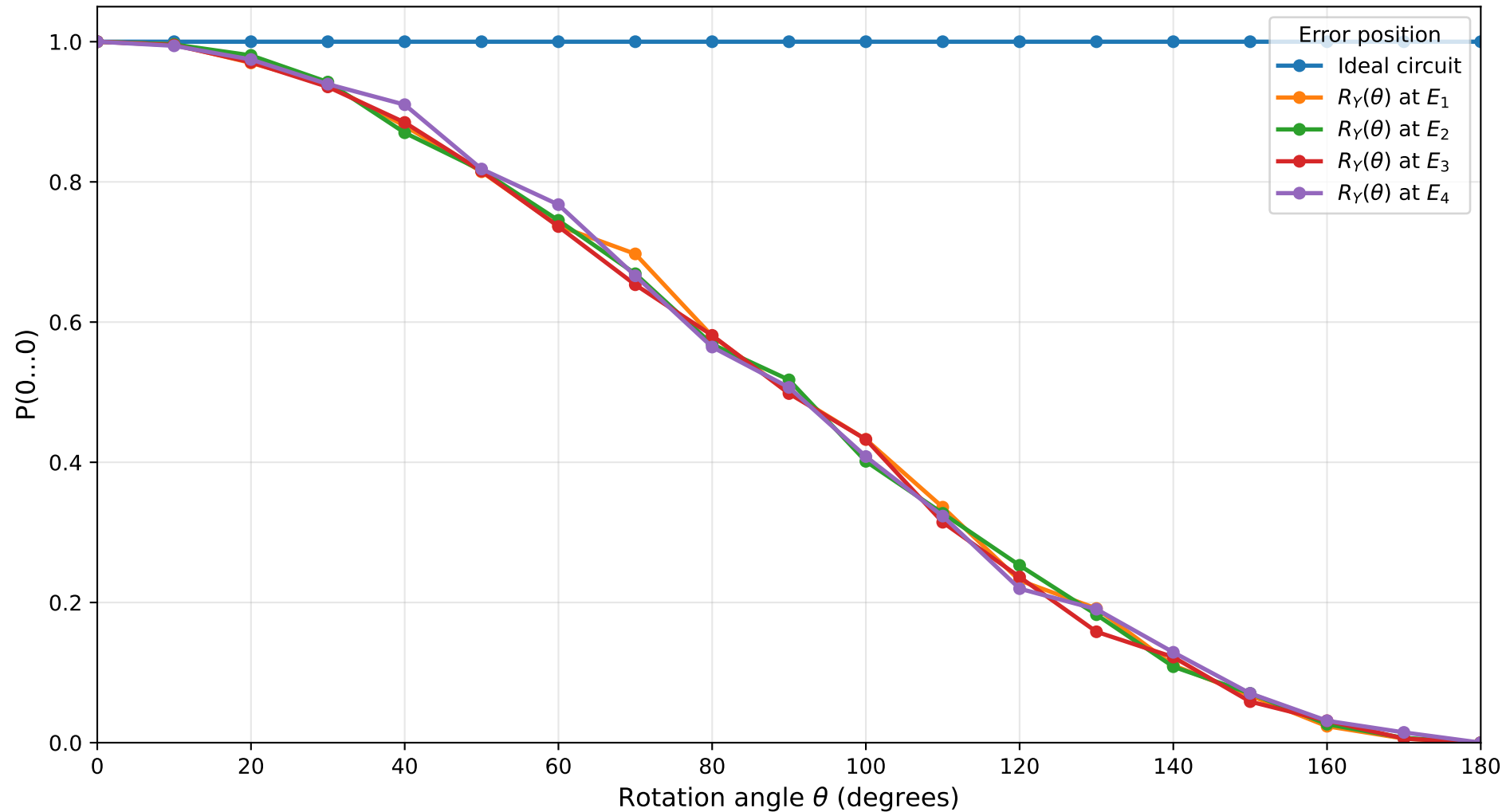
Probability under Y-Axis Rotation Errors Constant 0, n=3 , target qubit=2, shots=1024
