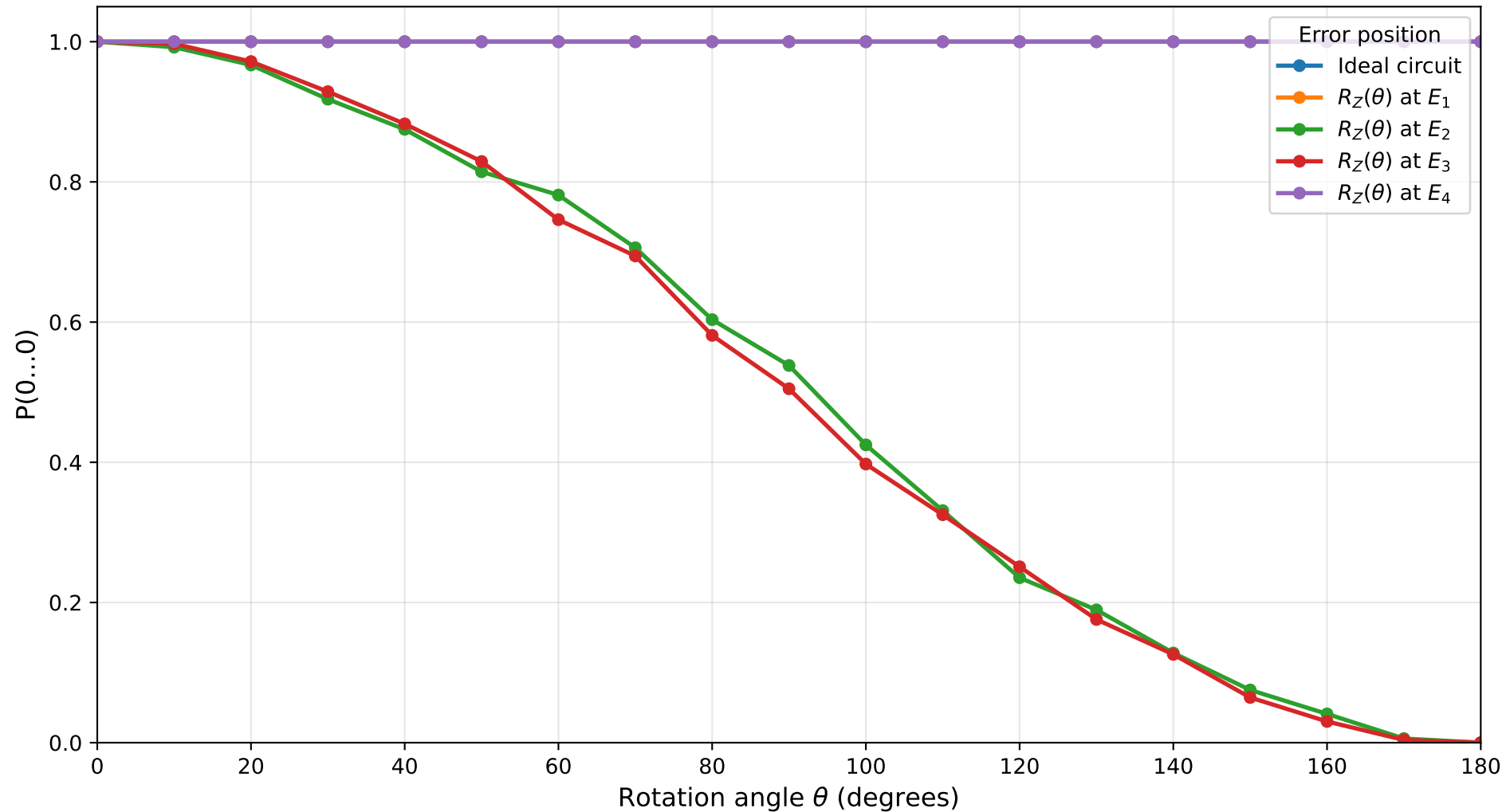
Probability under Z-Axis Rotation Errors Constant 0, n=3 , target qubit=2, shots=1024
