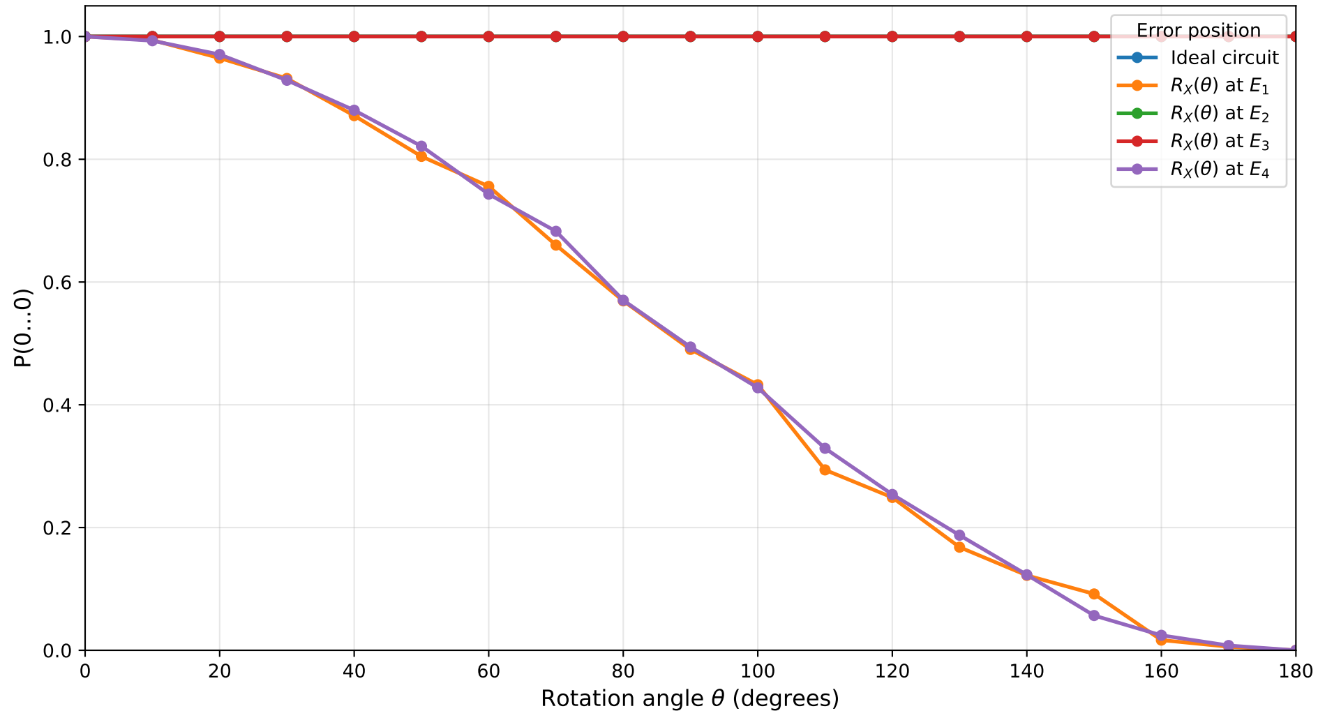
Probability under X-Axis Rotation Errors Constant 0, n=5 , target qubit=4, shots=1024
