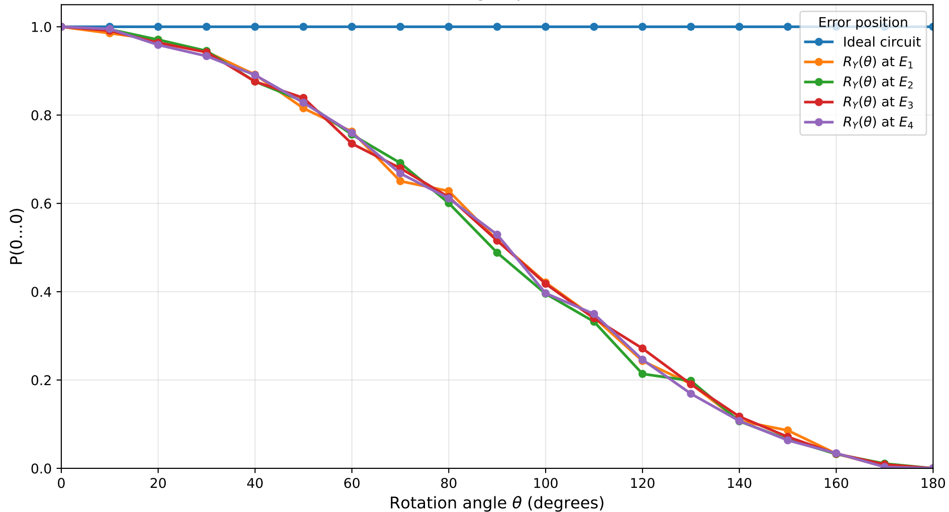
Probability under Y-Axis Rotation Errors Constant 0, n=5 , target qubit=4, shots=1024
