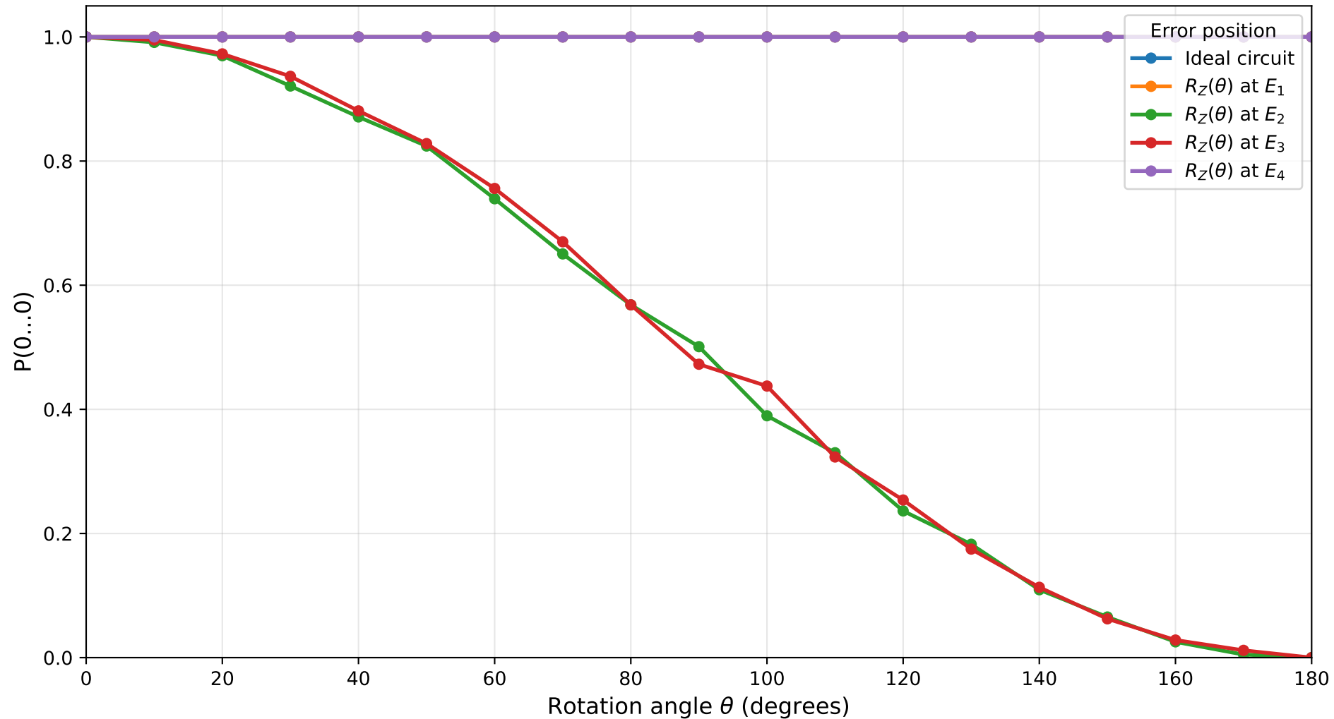
Probability under Z-Axis Rotation Errors Constant 0, n=5, target qubit=4, shots=1024
